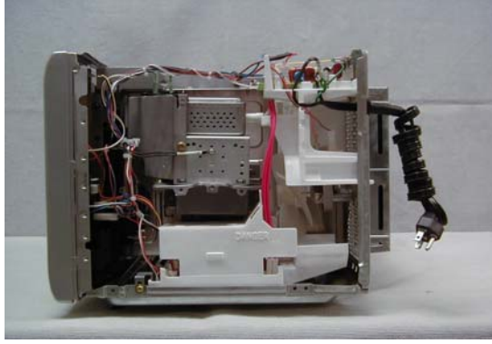
Exhibit 2-D2 Right side view, No enclosure NN-G464MFR
