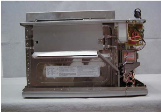
Exhibit 2-F2 Top view, No enclosure NN-G464MFR
