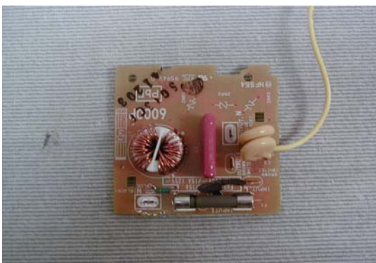
Exhibit 2-I View of Power Line Filter
