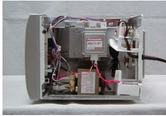
Exhibit 2-D2 Right Side View No Enclosure NN-G354MFR
