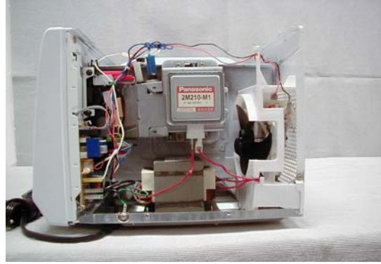
Exhibit 2-D2 Right side view, No enclosure NN-S335WF
