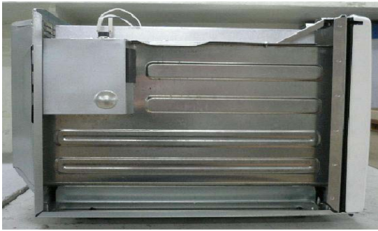
Exhibit 2-C2: Left Side View of Model MCEW With Enclosure Removed
