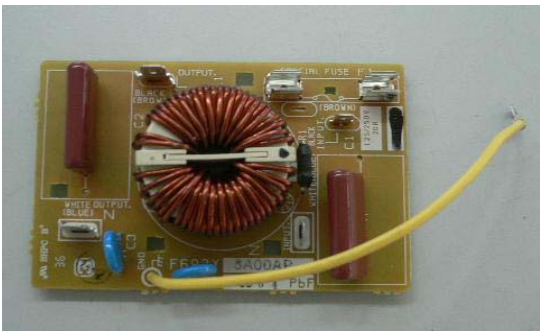
Exhibit 2-I: View of Power Line Filter
