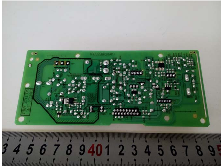
EUT –Controller Board Bottom Components View
