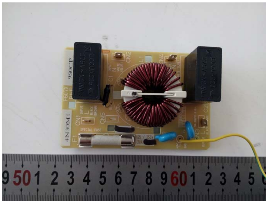
EUT –Filter Board Components View
