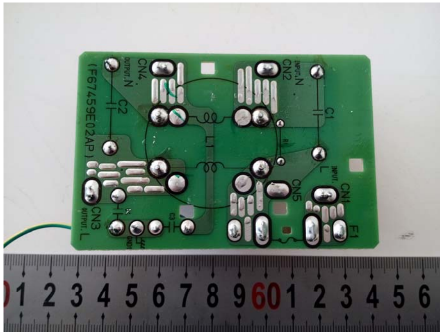
EUT –Filter Board Circuits View
