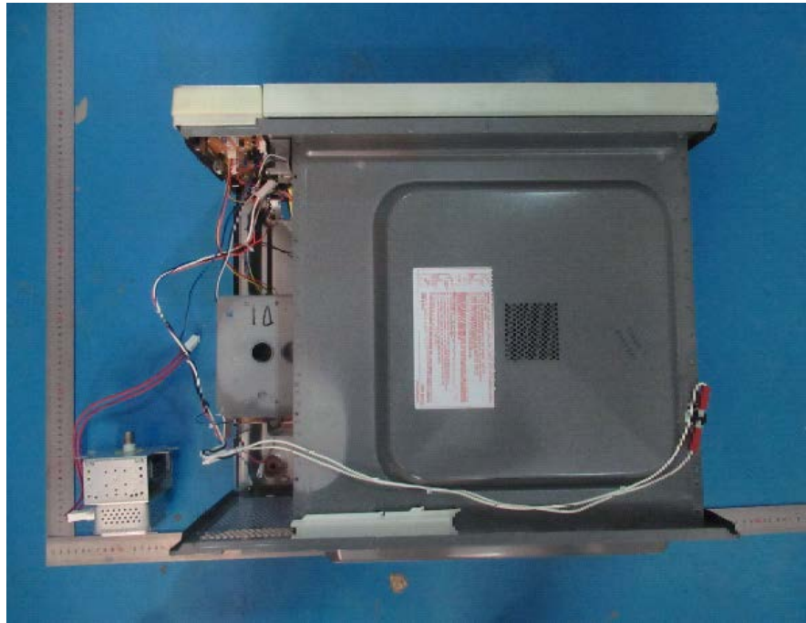
EUT – Cover off View -8
