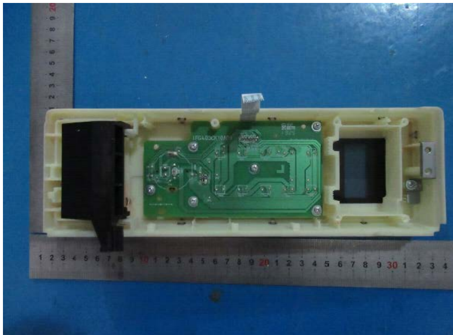
EUT- Cover off View -18
