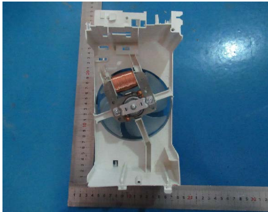
EUT – Cover off View -6
