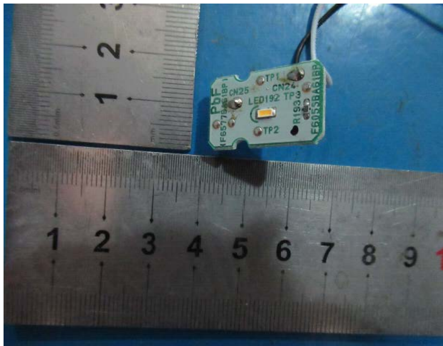
EUT- PCB-3 Bottom View
