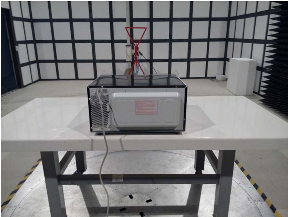
Radiated Emissions - Rear View (30 MHz – 1 GHz)
