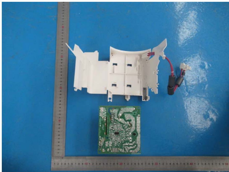
EUT- Cover off View -15
