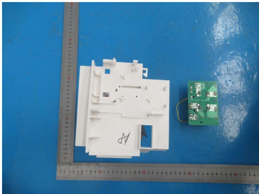
EUT- Cover off View -13
