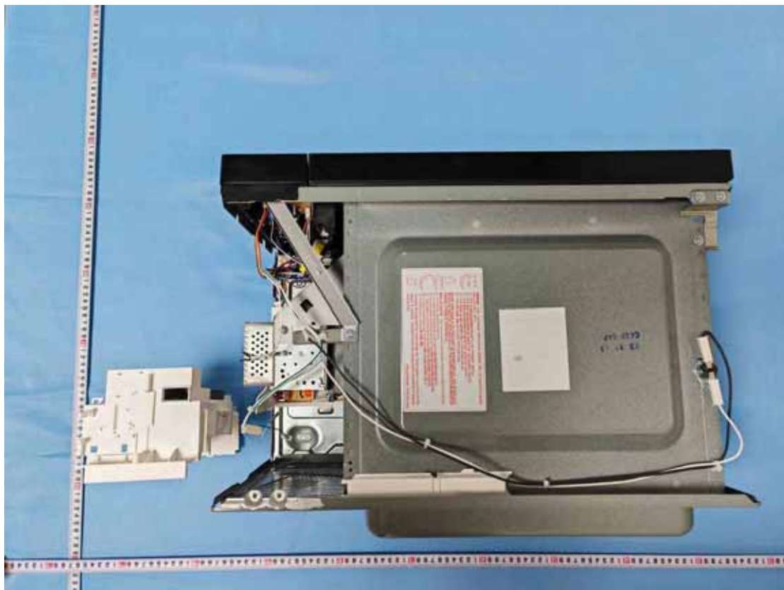
Figure 19 Cover Off View-10
