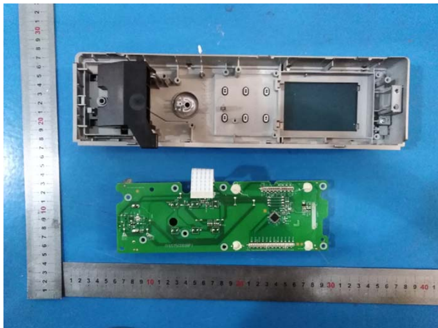
EUT- Cover off View -21
