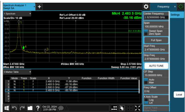
Bandedge CH39 (Upper)
