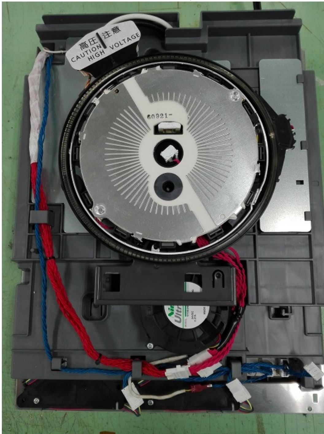
Overall view of KY-MK3500 induction heater cook top (internal).
