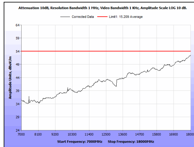
Plot 27. Radiated Spurious Emissions, Mid Channel, Antenna 1, 7 GHz – 18 GHz, Average
