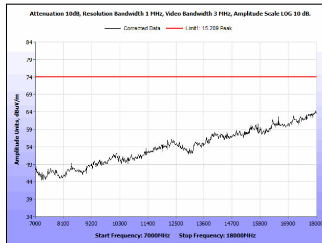
Plot 40. Radiated Spurious Emissions, Mid Channel, Antenna 2, 7 GHz – 18 GHz, Peak
