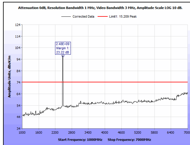
Plot 30. Radiated Spurious Emissions, High Channel, Antenna 1, 1 GHz – 7 GHz, Peak
