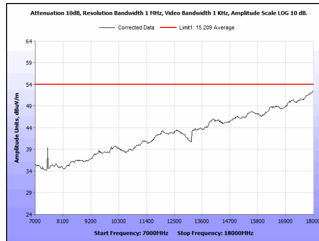
Plot 39. Radiated Spurious Emissions, Mid Channel, Antenna 2, 7 GHz – 18 GHz, Average
