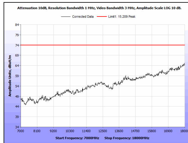
Plot 28. Radiated Spurious Emissions, Mid Channel, Antenna 1, 7 GHz – 18 GHz, Peak
