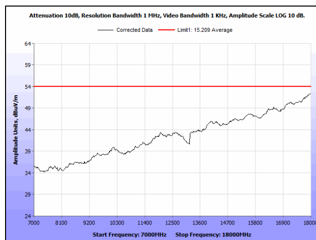
Plot 35. Radiated Spurious Emissions, Low Channel, Antenna 2, 7 GHz – 18 GHz, Average
