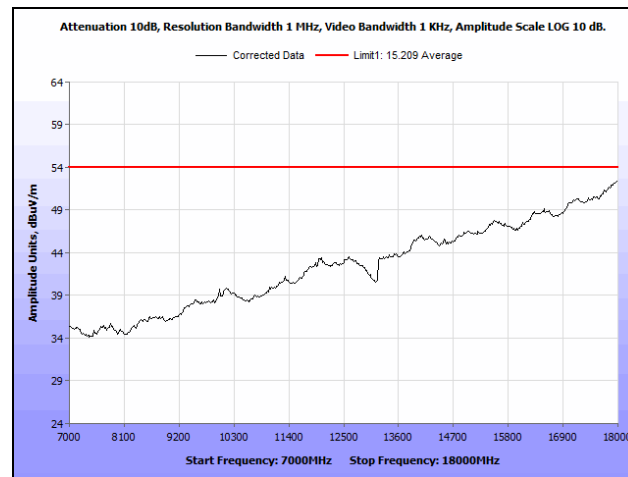
Plot 43. Radiated Spurious Emissions, High Channel, Antenna 2, 7 GHz – 18 GHz, Average
