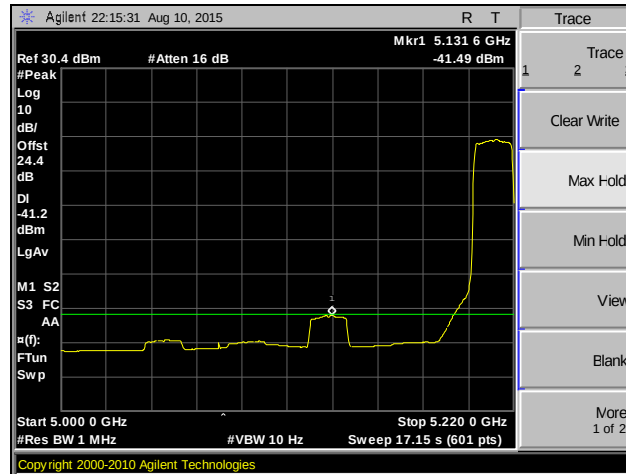
Plot 134. Band Edge, 802.11ac 20 MHz, MIMO, Channel 42, Average
