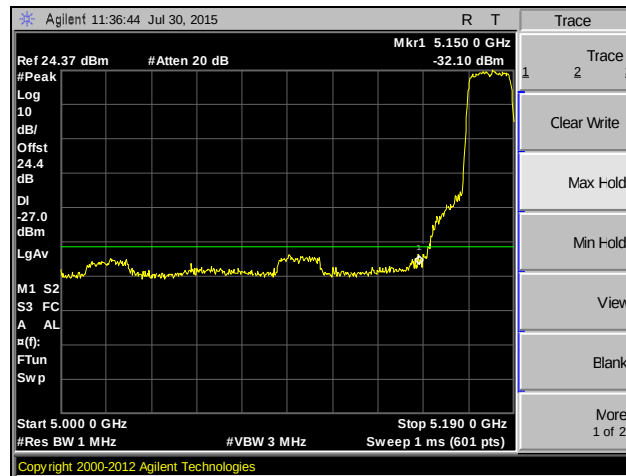
Plot 129. Band Edge, 802.11ac 20 MHz, MIMO, Channel 36, Peak
