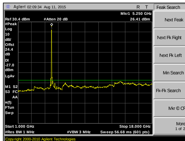
Plot 80. Spurious Emissions, 802.11ac 20 MHz, MIMO, High Channel
