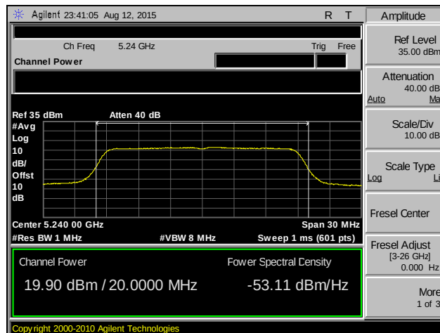
Plot 35. Conducted Output Power, 802.11n 20 MHz, MIMO, Channel 48
