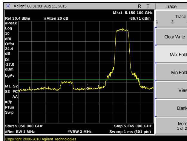
Plot 173. Band Edge, 802.11n 20 MHz, MIMO, Channel 40, Peak
