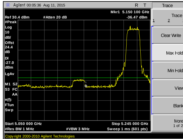
Plot 137. Band Edge, 802.11ac 20 MHz, MIMO, Channel 44, Peak
