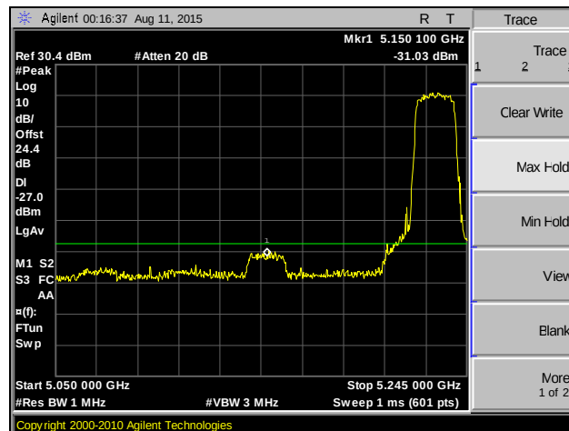
Plot 179. Band Edge, 802.11n 20 MHz, MIMO, Channel 46, Peak
