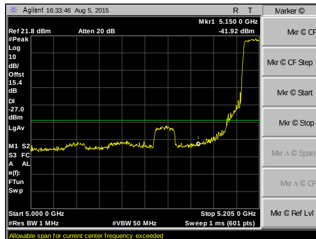
Plot 147. Band Edge, 802.11ac 20 MHz, SISO, Channel 40, Peak
