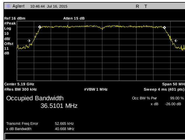
Plot 13. Occupied Bandwidth, 802.11n 40 MHz, 5190 MHz, Port 1
