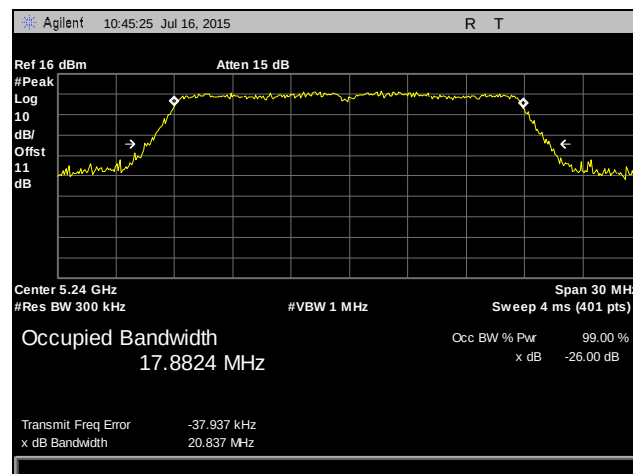
Plot 6. Occupied Bandwidth, 802.11ac 20 MHz, 5240 MHz, Port 1
