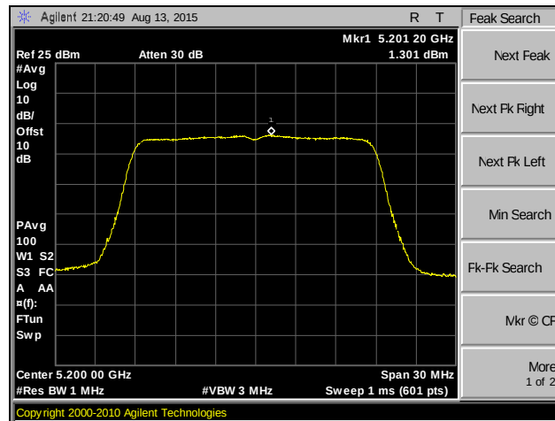
Plot 50. Peak Power Spectral Density, 802.11ac 20 MHz, MIMO, Channel 40
