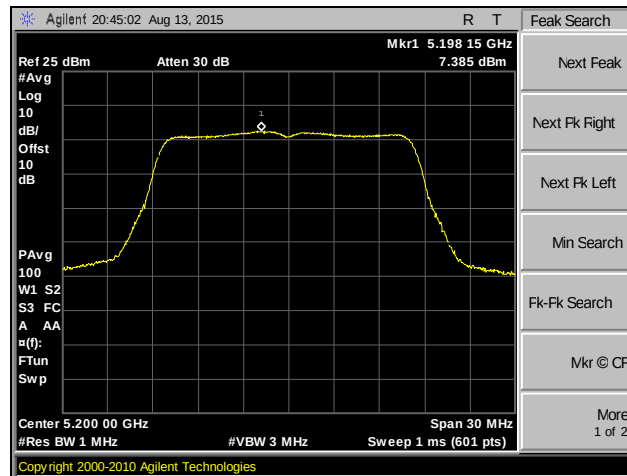
Plot 47. Peak Power Spectral Density, 802.11a 20 MHz, SISO, Channel 40
