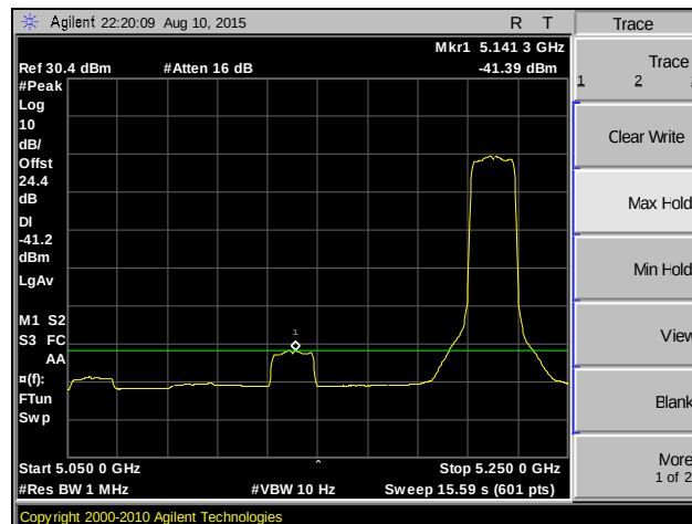
Plot 108. Band Edge, 802.11a 20 MHz, MIMO, Channel 44, Average
