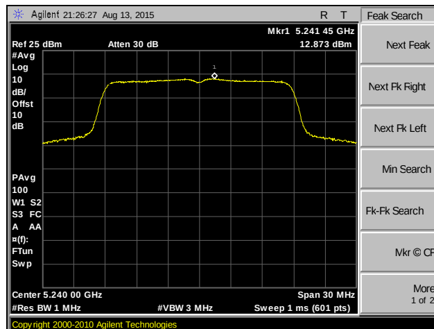
Plot 66. Peak Power Spectral Density, 802.11n 20 MHz, SISO, Channel 48
