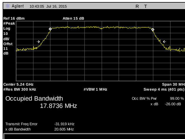
Plot 12. Occupied Bandwidth, 802.11n 20 MHz, 5240 MHz, Port 1
