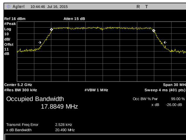
Plot 5. Occupied Bandwidth, 802.11ac 20 MHz, 5200 MHz, Port 1
