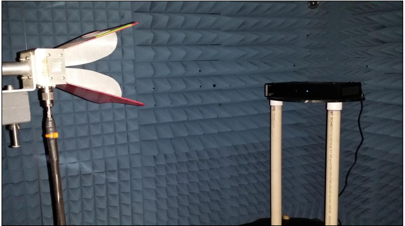
Photograph 1. Radiated Spurious Cabinet Emissions, Test Setup
