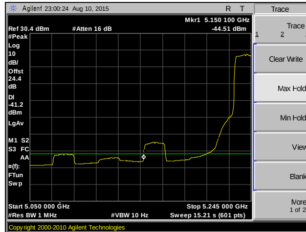
Plot 180. Band Edge, 802.11n 20 MHz, MIMO, Channel 48, Average
