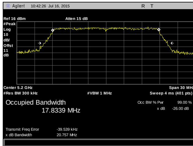
Plot 11. Occupied Bandwidth, 802.11n 20 MHz, 5200 MHz, Port 1
