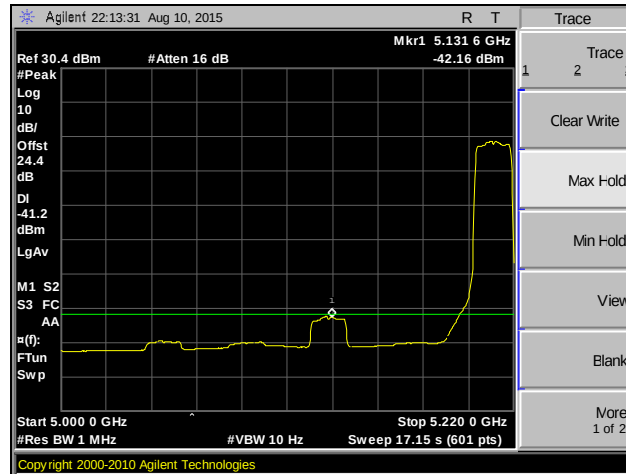
Plot 106. Band Edge, 802.11a 20 MHz, MIMO, Channel 42, Average
