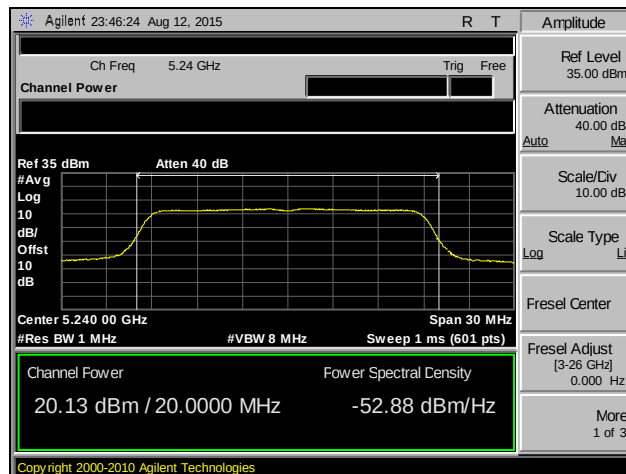
Plot 23. Conducted Output Power, 802.11ac 20 MHz, MIMO, Channel 48
