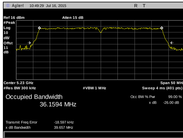
Plot 8. Occupied Bandwidth, 802.11ac 40 MHz, 5230 MHz, Port 1
