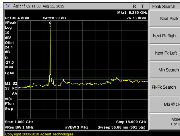
Plot 74. Spurious Emissions, 802.11a 20 MHz, MIMO, High Channel
