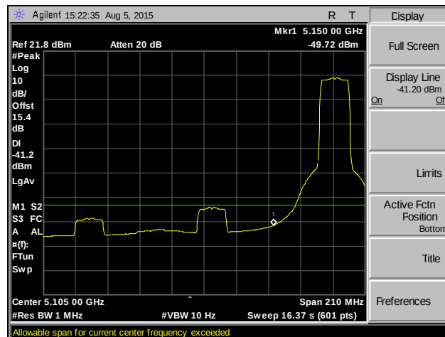
Plot 184. Band Edge, 802.11n 20 MHz, SISO, Channel 38, Average
