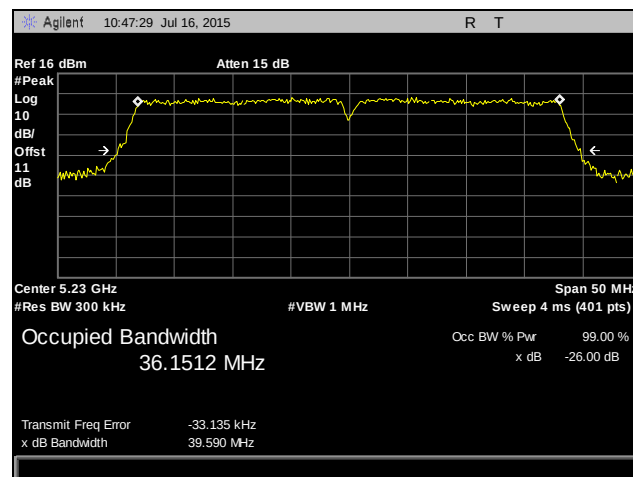
Plot 14. Occupied Bandwidth, 802.11n 40 MHz, 5230 MHz, Port 1
