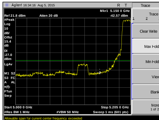
Plot 187. Band Edge, 802.11n 20 MHz, SISO, Channel 40, Peak
