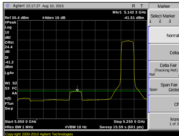
Plot 136. Band Edge, 802.11ac 20 MHz, MIMO, Channel 44, Average
