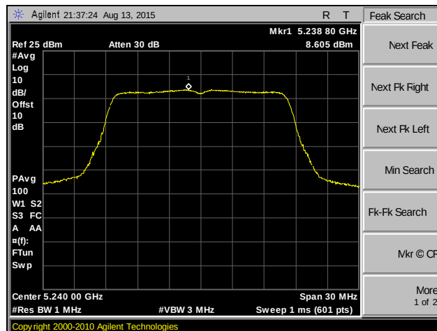
Plot 45. Peak Power Spectral Density, 802.11a 20 MHz, MIMO, Channel 48
