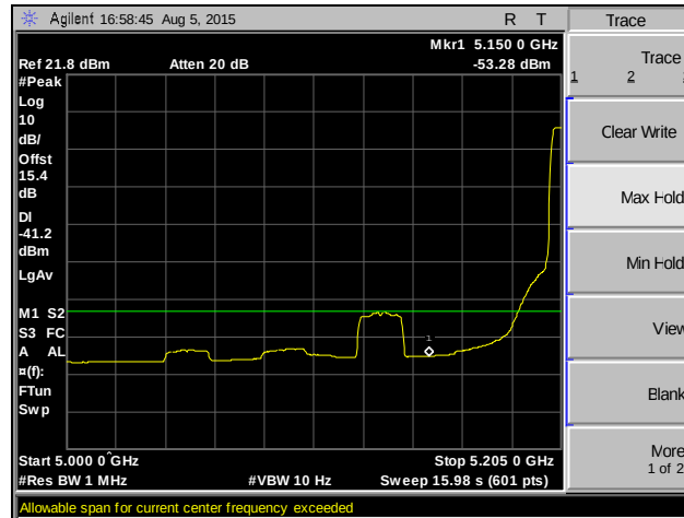
Plot 188. Band Edge, 802.11n 20 MHz, SISO, Channel 42, Average
