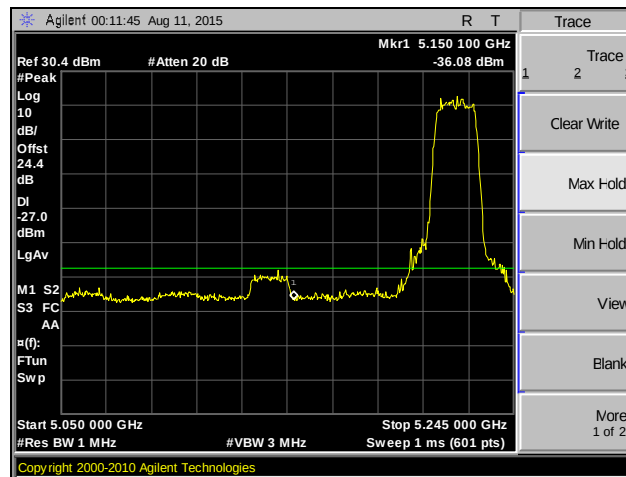
Plot 109. Band Edge, 802.11a 20 MHz, MIMO, Channel 44, Peak
