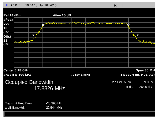
Plot 4. Occupied Bandwidth, 802.11ac 20 MHz, 5180 MHz, Port 1
