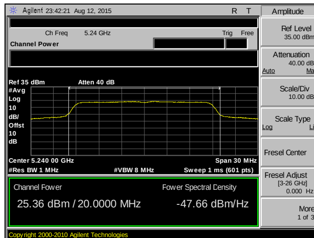
Plot 38. Conducted Output Power, 802.11n 20 MHz, SISO, Channel 48
