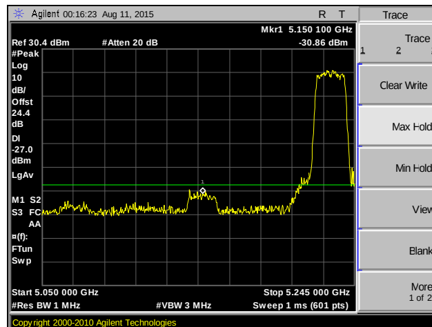
Plot 139. Band Edge, 802.11ac 20 MHz, MIMO, Channel 46, Peak
