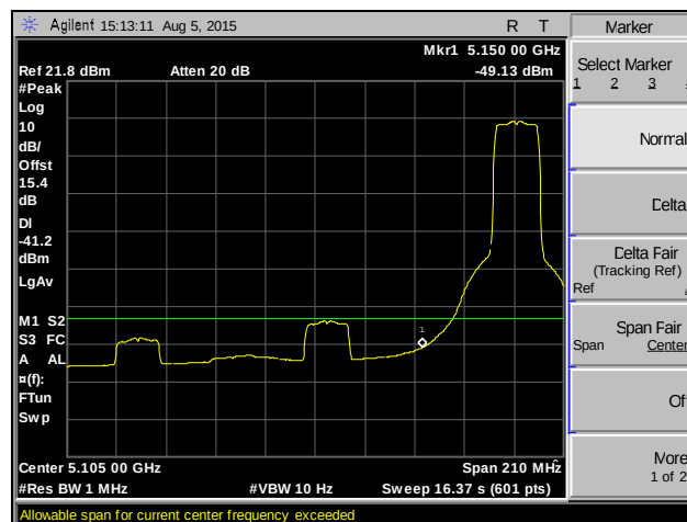
Plot 144. Band Edge, 802.11ac 20 MHz, SISO, Channel 38, Average
