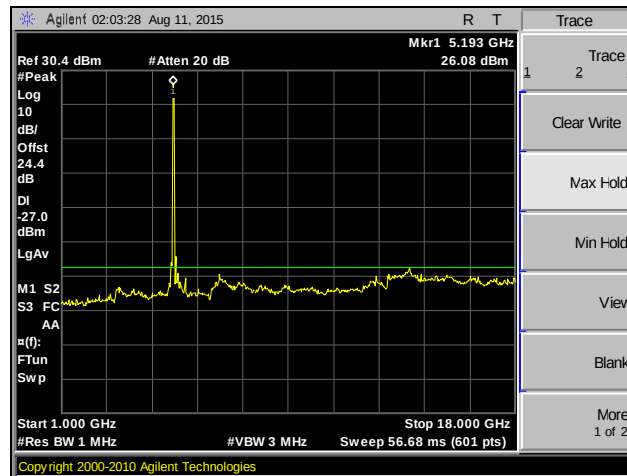
Plot 73. Spurious Emissions, 802.11a 20 MHz, MIMO, Mid Channel
