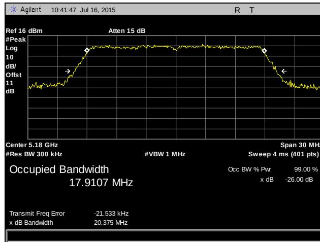
Plot 10. Occupied Bandwidth, 802.11n 20 MHz, 5180 MHz, Port 1
