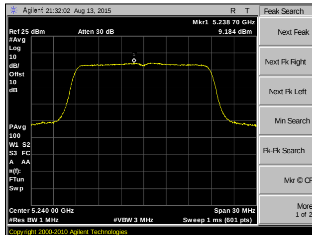
Plot 51. Peak Power Spectral Density, 802.11ac 20 MHz, MIMO, Channel 48
