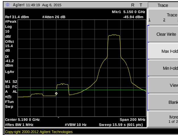
Plot 154. Band Edge, 802.11ac 20 MHz, SISO, Channel 48, Average
