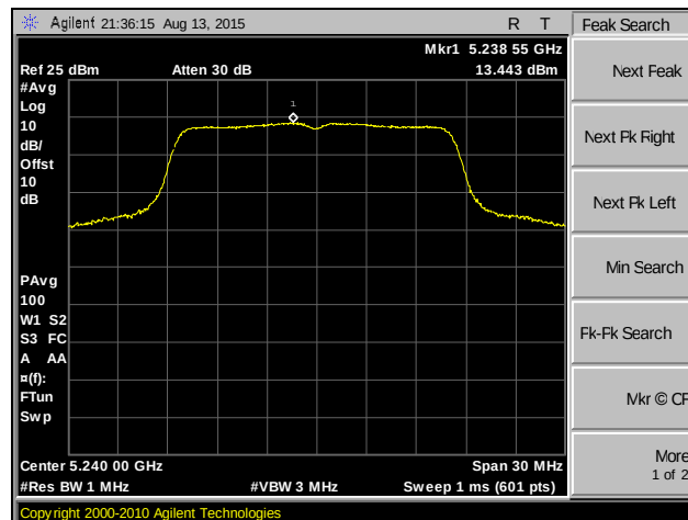
Plot 48. Peak Power Spectral Density, 802.11a 20 MHz, SISO, Channel 48
