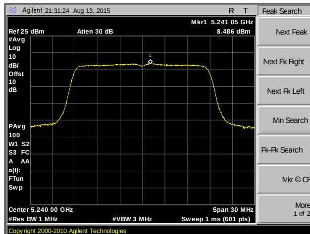
Plot 63. Peak Power Spectral Density, 802.11n 20 MHz, MIMO, Channel 48
