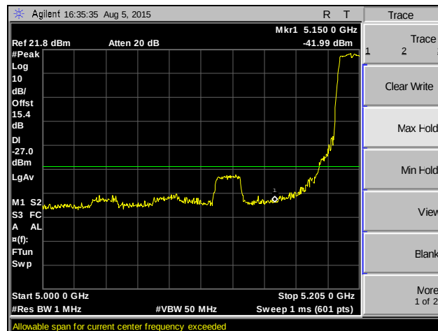
Plot 119. Band Edge, 802.11a 20 MHz, SISO, Channel 40, Peak
