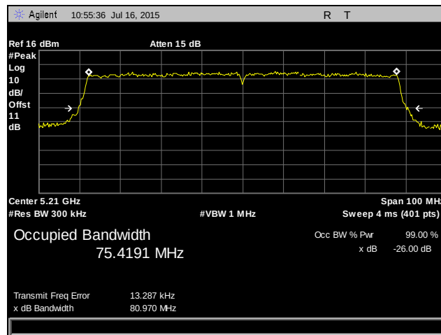
Plot 9. Occupied Bandwidth, 802.11ac 80 MHz, 5210 MHz, Port 1
