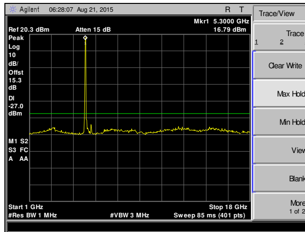
Plot 244. Spurious Emissions, 802.11n 20 MHz, Channel 60, SISO
