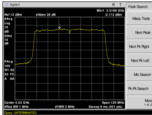
Plot 169. Peak Power Spectral Density, 802.11ac 80 MHz, Channel 100, SISO
