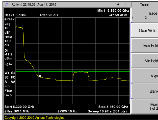
Plot 328. Band Edge, 802.11n 20 MHz, Channel 64, SISO
