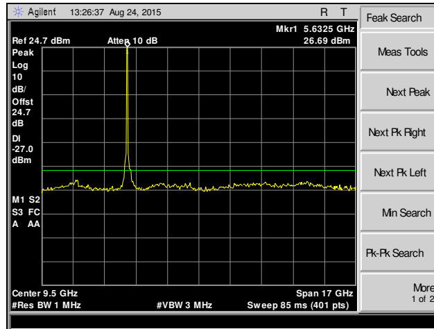
Plot 216. Spurious Emissions, 802.11n 40 MHz, Channel 116, MIMO
