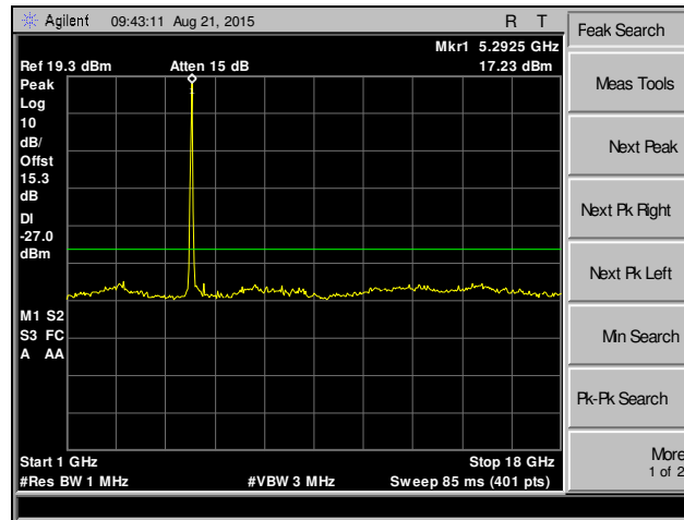
Plot 250. Spurious Emissions, 802.11n 40 MHz, Channel 52, SISO
