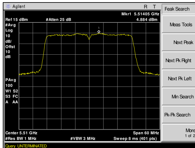
Plot 181. Peak Power Spectral Density, 802.11n 40 MHz, Channel 100, SISO
