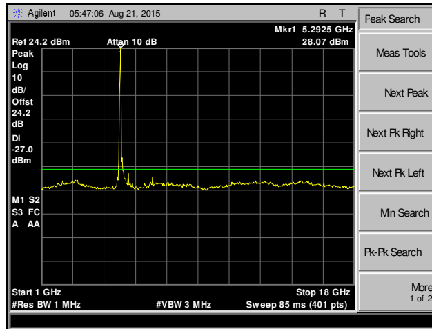
Plot 185. Spurious Emissions, 802.11a, Channel 52, MIMO
