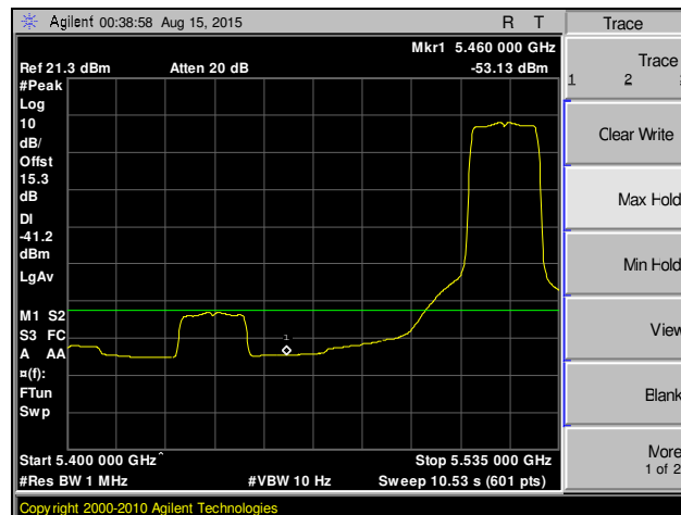
Plot 330. Band Edge, 802.11n 20 MHz, Channel 104, SISO
