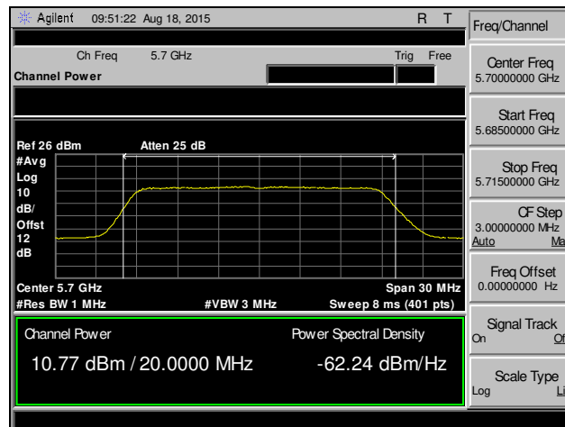
Plot 67. RF Output Power, 802.11n 20 MHz, Channel 140, MIMO
