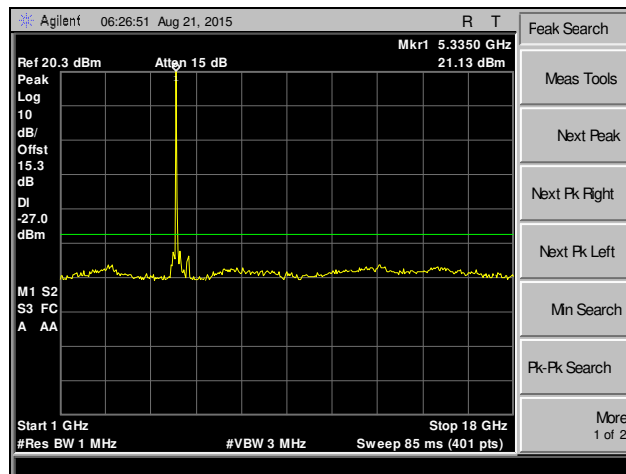
Plot 245. Spurious Emissions, 802.11n 20 MHz, Channel 64, SISO
