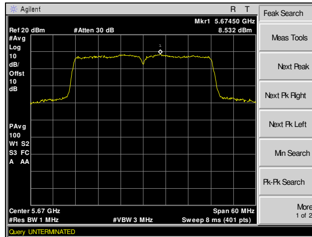
Plot 183. Peak Power Spectral Density, 802.11n 40 MHz, Channel 132, SISO
