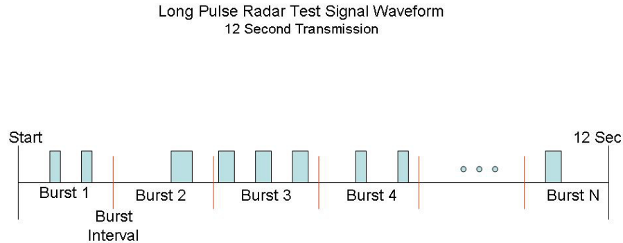
Figure 4. Long Pulse Radar Test Signal Waveform
