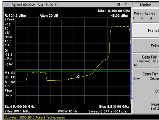
Plot 329. Band Edge, 802.11n 20 MHz, Channel 100, SISO
