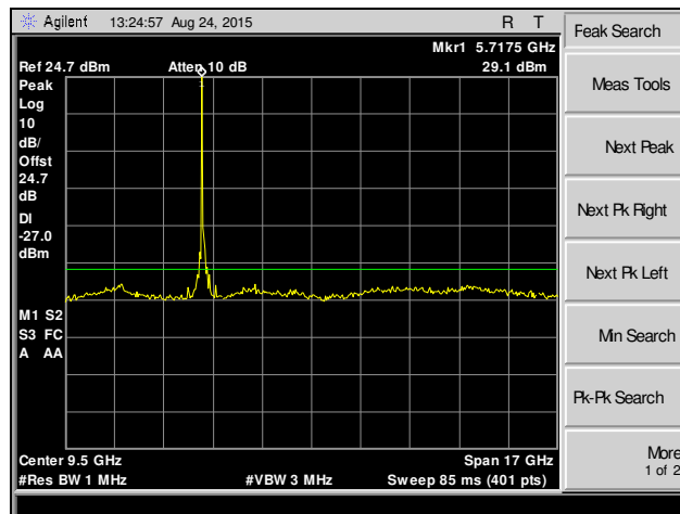
Plot 190. Spurious Emissions, 802.11a, Channel 140, MIMO
