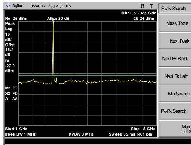
Plot 226. Spurious Emissions, 802.11ac 20 MHz, Channel 52, SISO
