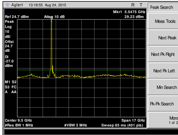
Plot 188. Spurious Emissions, 802.11a, Channel 100, MIMO
