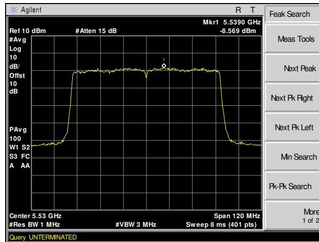
Plot 133. Peak Power Spectral Density, 802.11ac 80 MHz, Channel 100, MIMO
