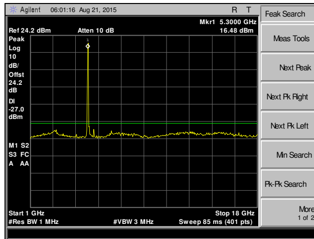
Plot 186. Spurious Emissions, 802.11a, Channel 60, MIMO
