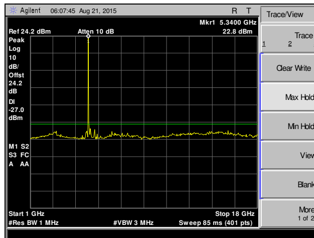
Plot 187. Spurious Emissions, 802.11a, Channel 64, MIMO
