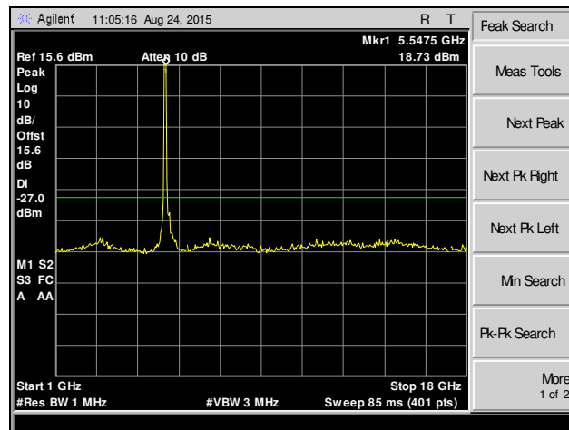
Plot 252. Spurious Emissions, 802.11n 40 MHz, Channel 100, SISO
