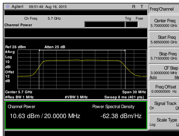
Plot 50. RF Output Power, 802.11ac 20 MHz, Channel 140, MIMO
