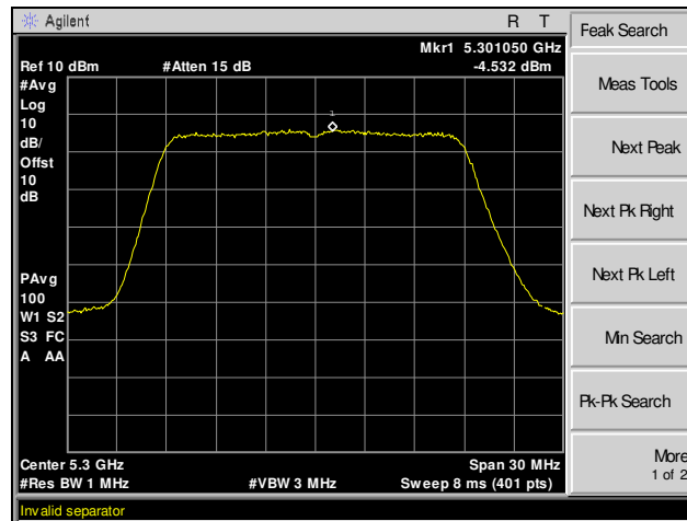
Plot 120. Peak Power Spectral Density, 802.11ac 20 MHz, Channel 60, MIMO
