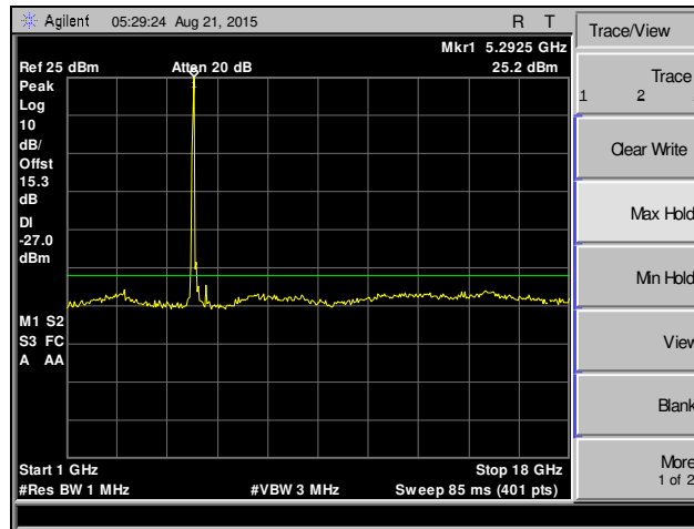
Plot 243. Spurious Emissions, 802.11n 20 MHz, Channel 52, SISO
