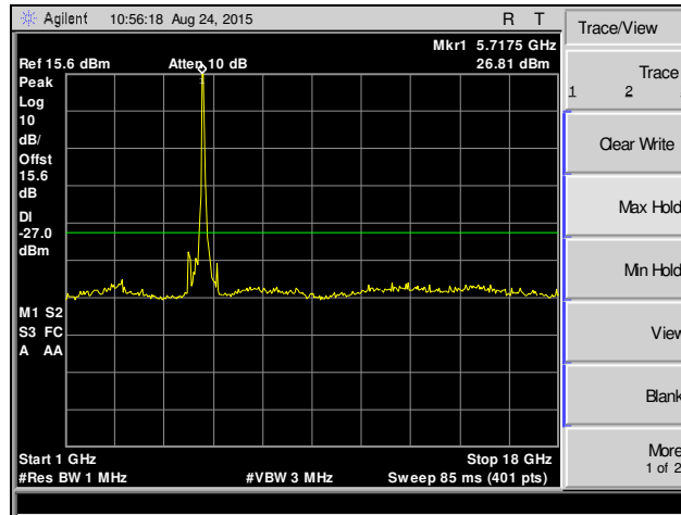
Plot 249. Spurious Emissions, 802.11n 20 MHz, Channel 144, SISO
