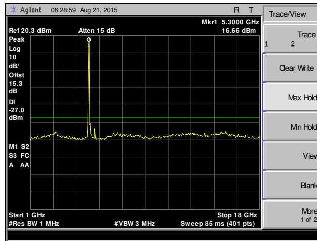
Plot 227. Spurious Emissions, 802.11ac 20 MHz, Channel 60, SISO
