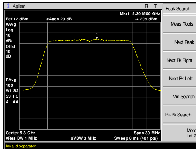
Plot 137. Peak Power Spectral Density, 802.11n 20 MHz, Channel 60, MIMO
