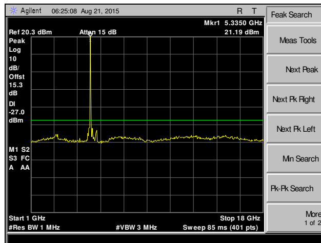
Plot 228. Spurious Emissions, 802.11ac 20 MHz, Channel 64, SISO
