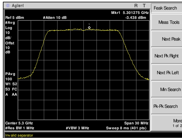
Plot 113. Peak Power Spectral Density, 802.11a, Channel 60, MIMO
