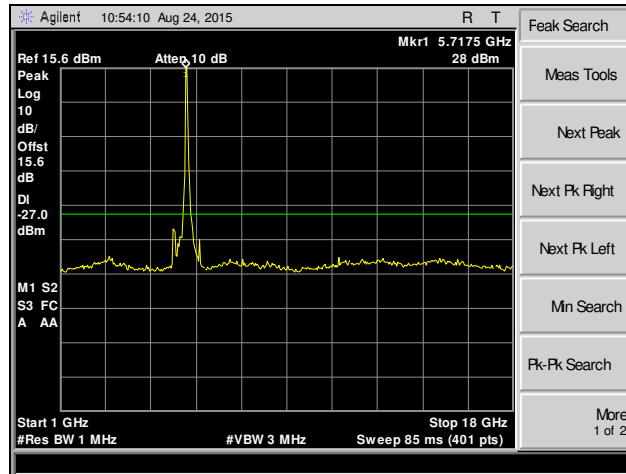
Plot 225. Spurious Emissions, 802.11a, Channel 144, SISO
