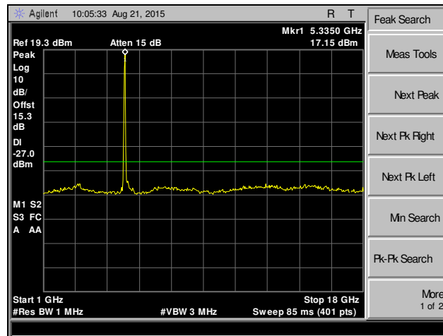
Plot 251. Spurious Emissions, 802.11n 40 MHz, Channel 60, SISO
