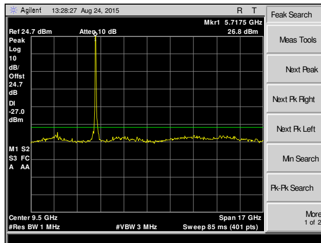
Plot 218. Spurious Emissions, 802.11n 40 MHz, Channel 140, MIMO
