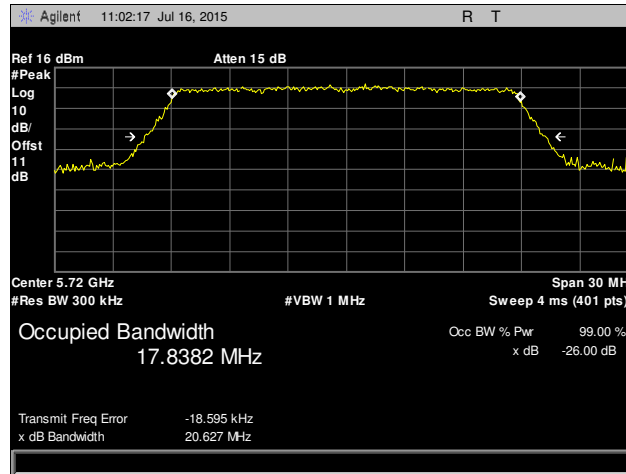
Plot 32. Occupied Bandwidth, 802.11n 20 MHz, 5720 MHz, Port 1
