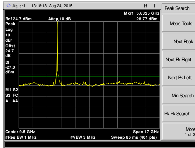
Plot 189. Spurious Emissions, 802.11a, Channel 120, MIMO
