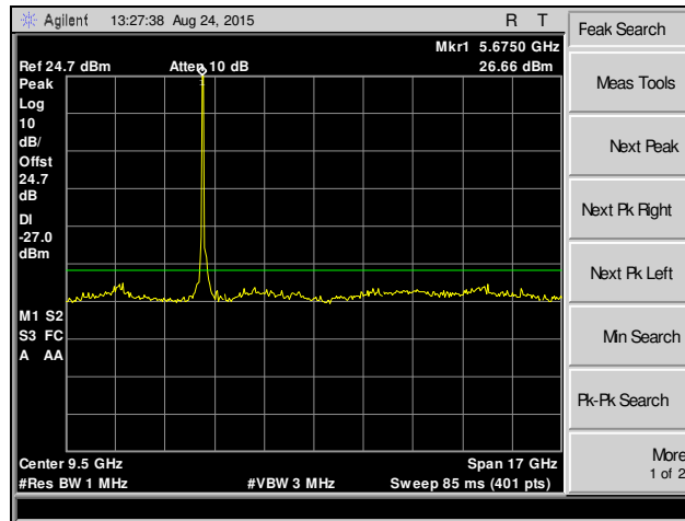
Plot 217. Spurious Emissions, 802.11n 40 MHz, Channel 132, MIMO
