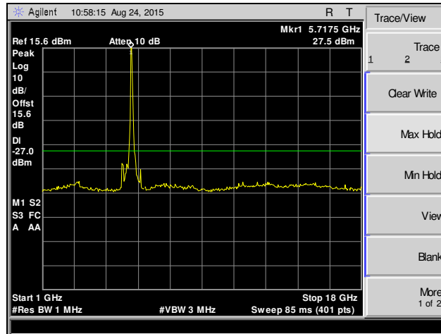
Plot 232. Spurious Emissions, 802.11ac 20 MHz, Channel 144, SISO
