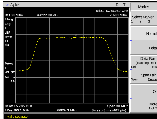
Plot 55. Peak Power Spectral Density, Channel 157, 802.11ac 20 MHz, SISO
