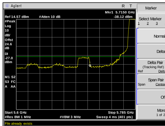
Plot 151. Band Edge, Channel 157, 802.11n 20 MHz, MIMO
