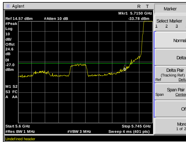
Plot 150. Band Edge, Channel 149, 802.11n 20 MHz, MIMO
