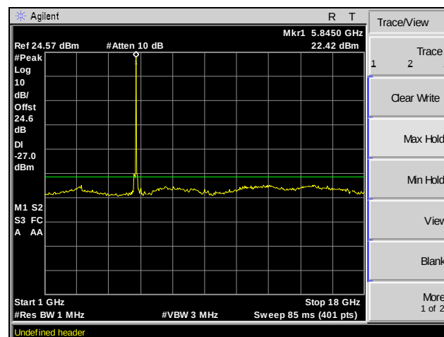
Plot 90. Spurious Emissions, Channel 165, 802.11ac 20 MHz, MIMO, 1 GHz – 18 GHz
