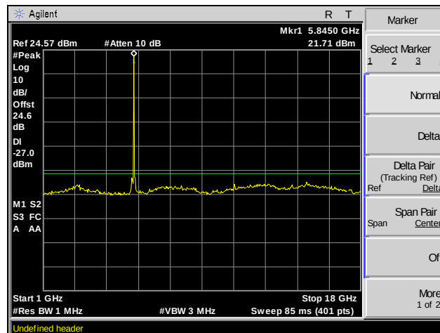
Plot 78. Spurious Emissions, Channel 165, 802.11a 20 MHz, MIMO, 1 GHz – 18 GHz
