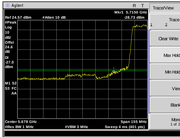
Plot 156. Band Edge, Channel 149, 802.11n 40 MHz, MIMO
