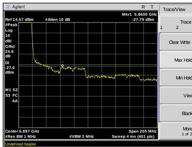
Plot 157. Band Edge, Channel 157, 802.11n 40 MHz, MIMO
