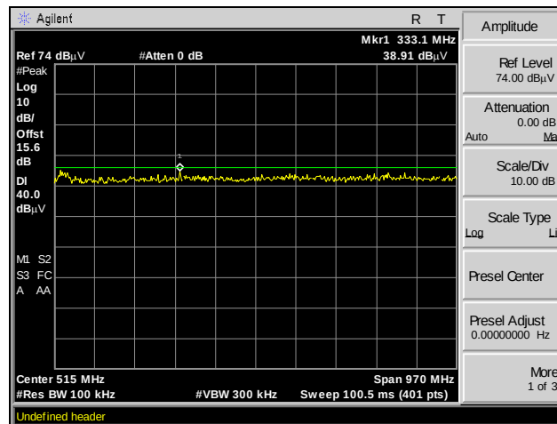
Plot 79. Spurious Emissions, Channel 149, 802.11a 20 MHz, SISO, 30 MHz – 1 GHz
