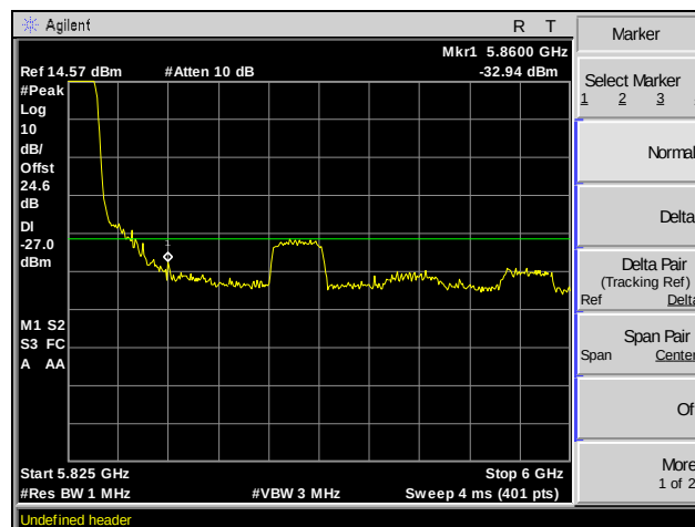
Plot 152. Band Edge, Channel 165, 802.11n 20 MHz, MIMO
