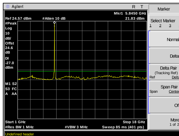
Plot 116. Spurious Emissions, Channel 165, 802.11n 20 MHz, MIMO, 1 GHz – 18 GHz
