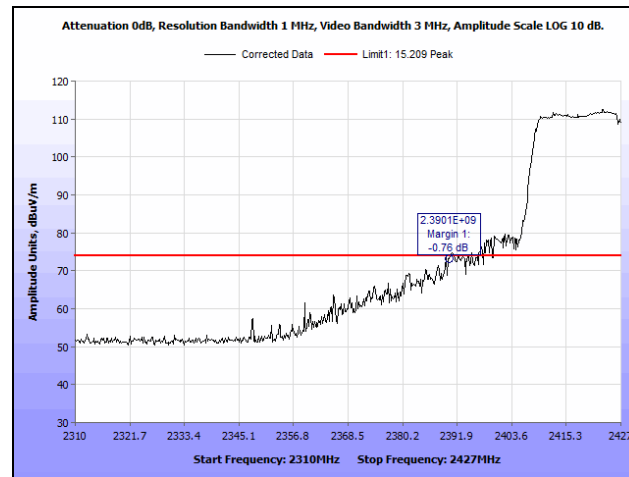
Plot 255. Radiated Restricted Band Edge, 2427 MHz, 802.11n 40 MHz, SISO, Peak
