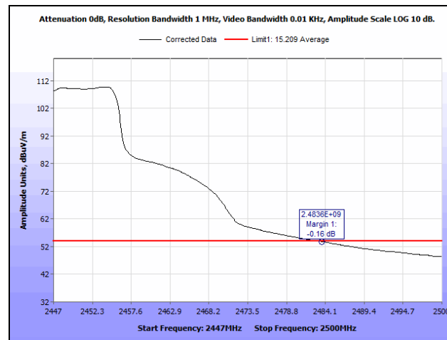
Plot 196. Radiated Restricted Band Edge, 2447 MHz, 802.11g, SISO, Average
