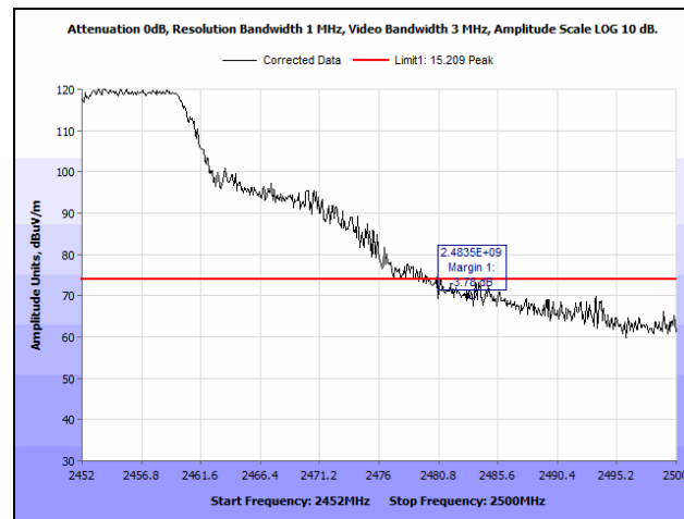
Plot 199. Radiated Restricted Band Edge, 2452 MHz, 802.11g, SISO, Peak
