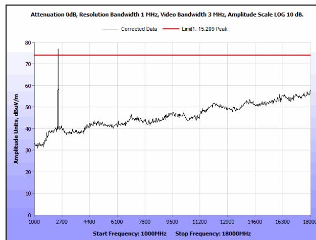
Plot 120. Radiated Spurious Emissions, High Channel, 802.11g, 1 GHz – 18 GHz, Peak, MIMO
