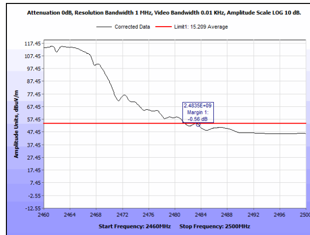
Plot 176. Radiated Restricted Band Edge, 2462 MHz, 802.11b, SISO, Average
