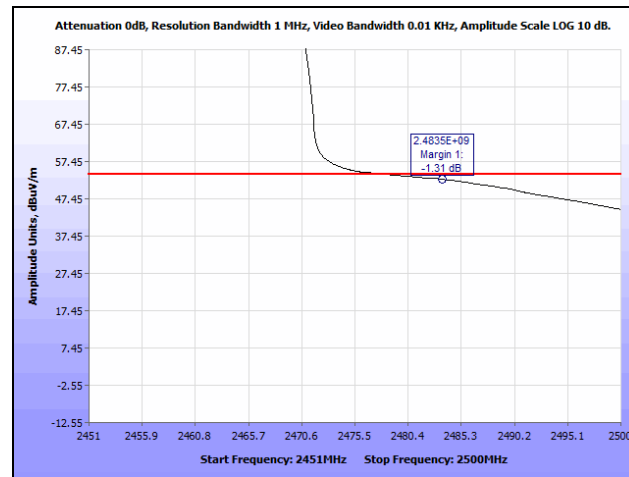
Plot 264. Radiated Restricted Band Edge, 2452 MHz, 802.11n 40 MHz, SISO, Average
