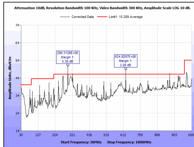
Plot 160. Radiated Spurious Emissions, Mid Channel, 802.11n 40 MHz, 30 MHz – 1 GHz, SISO
