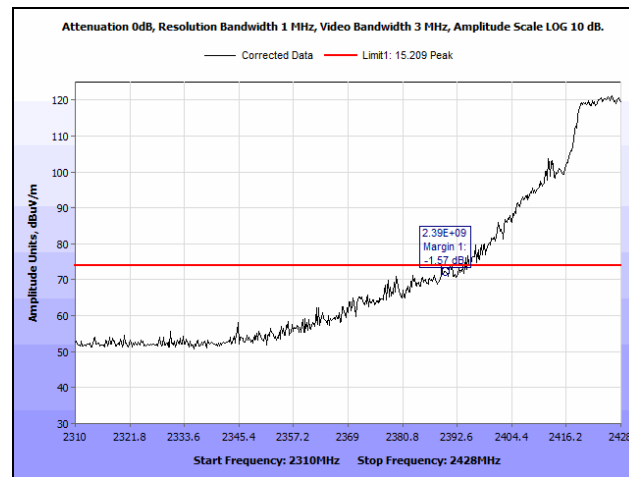
Plot 193. Radiated Restricted Band Edge, 2427 MHz, 802.11g, SISO, Peak
