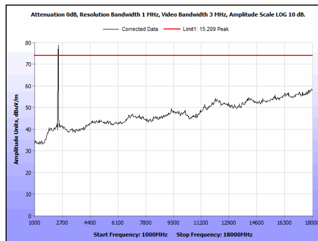
Plot 117. Radiated Spurious Emissions, Mid Channel, 802.11g, 1 GHz – 18 GHz, Peak, MIMO
