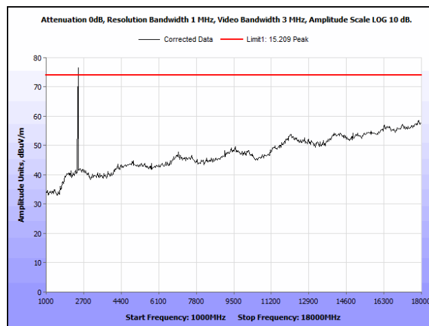
Plot 108. Radiated Spurious Emissions, Mid Channel, 802.11b, 1 GHz – 18 GHz, Peak, SISO
