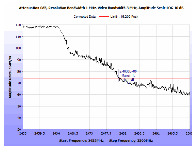
Plot 201. Radiated Restricted Band Edge, 2457 MHz, 802.11g, SISO, Peak
