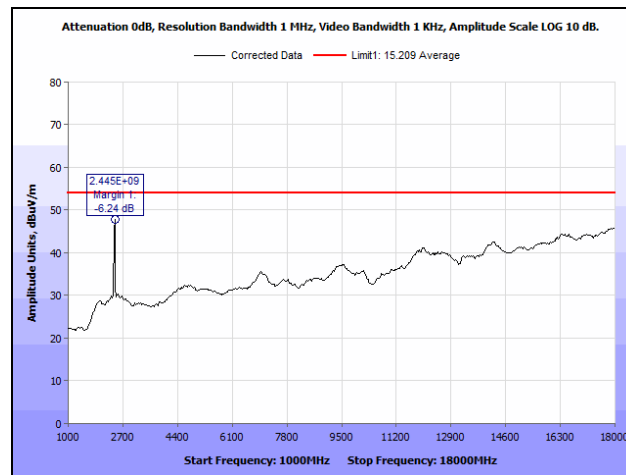
Plot 161. Radiated Spurious Emissions, Mid Channel, 802.11n 40 MHz, 1 GHz – 18 GHz, Average, SISO
