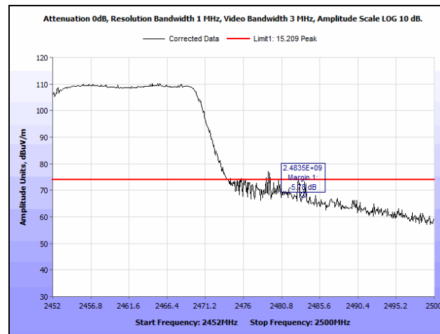
Plot 265. Radiated Restricted Band Edge, 2452 MHz, 802.11n 40 MHz, SISO, Peak
