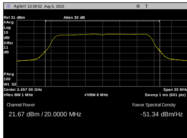
Plot 53. Peak Power Output, 2457 MHz, 802.11g, MIMO
