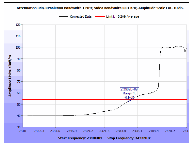
Plot 256. Radiated Restricted Band Edge, 2432 MHz, 802.11n 40 MHz, SISO, Average
