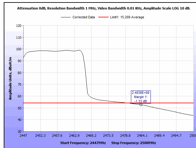
Plot 262. Radiated Restricted Band Edge, 2447 MHz, 802.11n 40 MHz, SISO, Average
