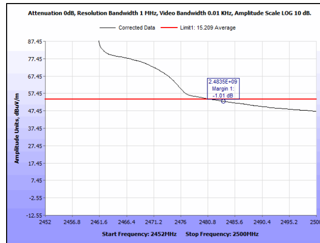
Plot 198. Radiated Restricted Band Edge, 2452 MHz, 802.11g, SISO, Average
