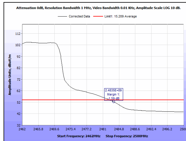
Plot 202. Radiated Restricted Band Edge, 2462 MHz, 802.11g, SISO, Average
