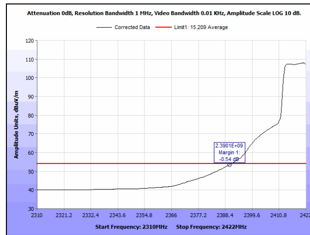
Plot 220. Radiated Restricted Band Edge, 2422 MHz, 802.11n 20 MHz, SISO, Average
