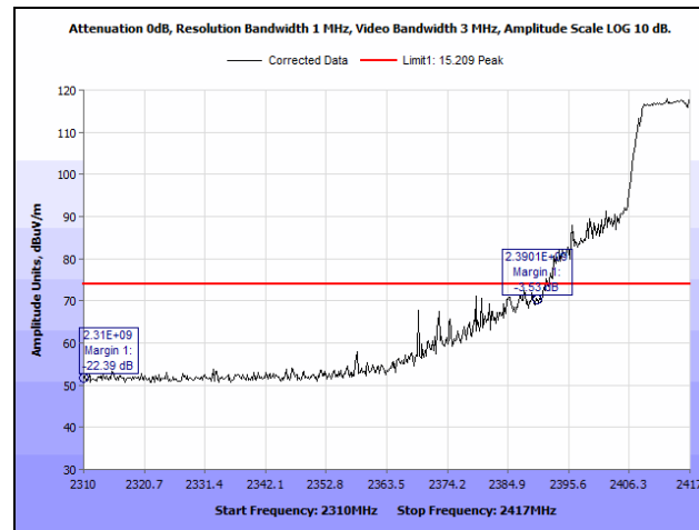
Plot 219. Radiated Restricted Band Edge, 2417 MHz, 802.11n 20 MHz, SISO, Peak
