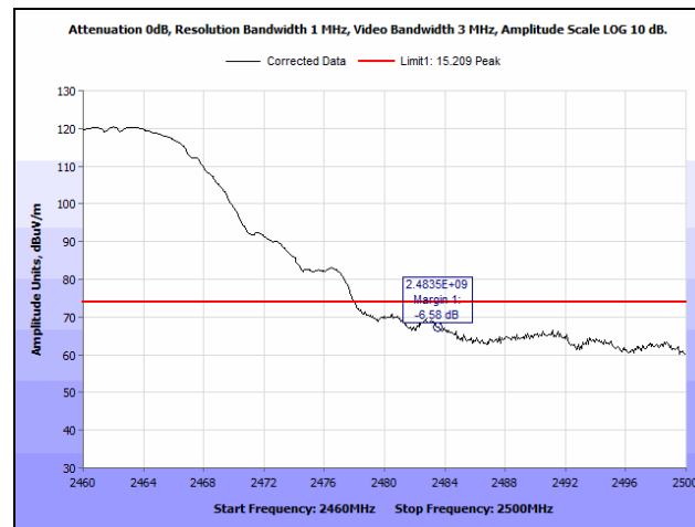
Plot 177. Radiated Restricted Band Edge, 2462 MHz, 802.11b, SISO, Peak
