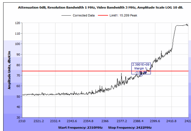
Plot 221. Radiated Restricted Band Edge, 2422 MHz, 802.11n 20 MHz, SISO, Peak
