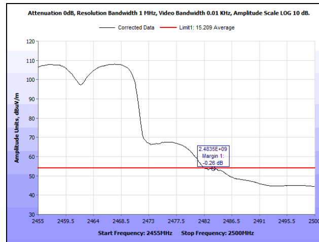
Plot 184. Radiated Restricted Band Edge, 2462 MHz, 802.11g, MIMO, Average
