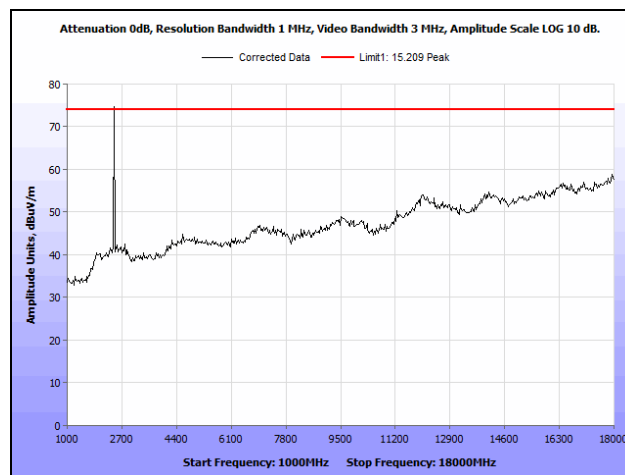
Plot 129. Radiated Spurious Emissions, High Channel, 802.11g, 1 GHz – 18 GHz, Peak, SISO
