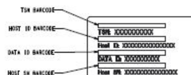
DETAIL B SCALE: 2:1 (REFER TO 267308-216 SPECIFICATION)
