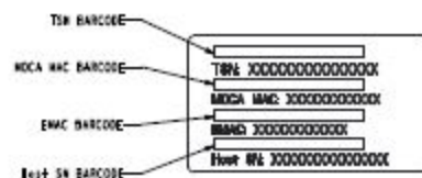
DETAIL A SCALE: 2:1 (REFER TO 207308-210 SPECIFICATION)
