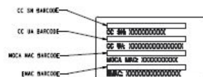
DETAIL C SCALE: 2:1 (REFER TO 207308-210 SPECIFICATION)
