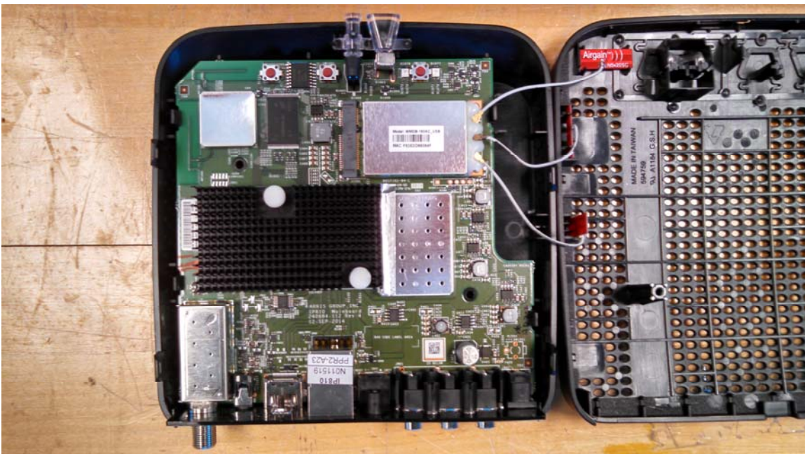
RADIO BOARD TOP
