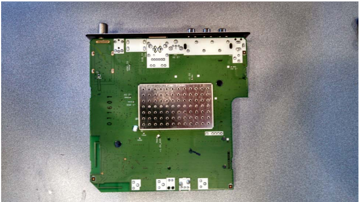
ARRIS IP815 INTERNAL BOTTOM
