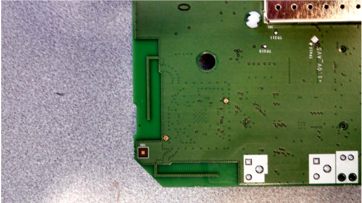
ARRIS IP815 INTERNAL RF4CE BOTTOM
