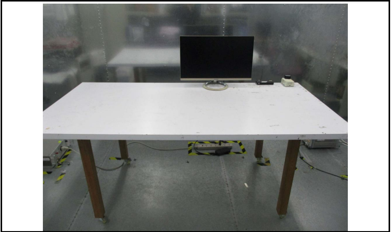
Conducted Emission Test (USB chip model GL852G)
