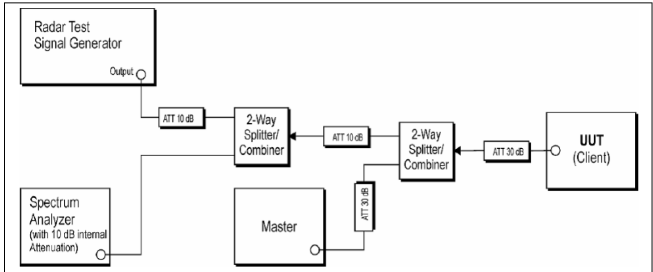
Figure 4. Test Setup Diagram
