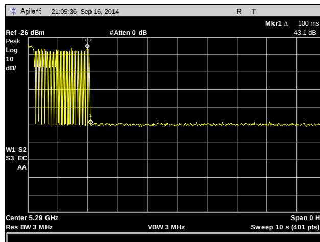
Plot 27. Channel Move Time, 10 second, Port JA1
