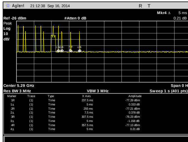
Plot 25. Channel Closing Transmission Time Aggregate, Port JA1
