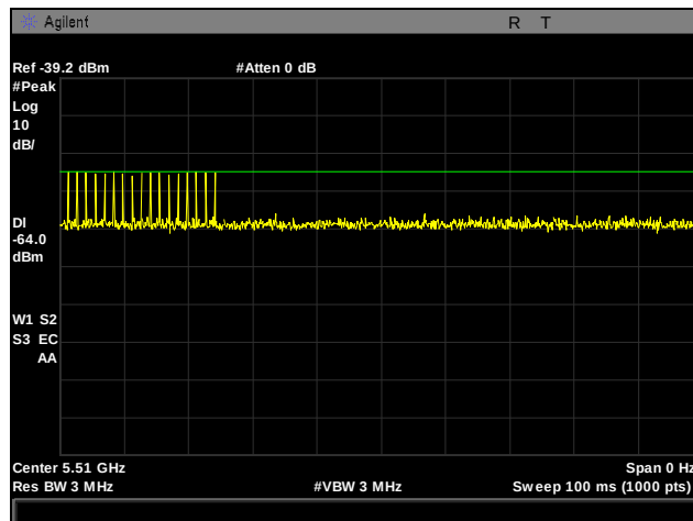
Plot 3. Radar Type 0 Calibration, 5510 MHz
