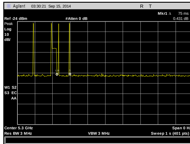
Plot 28. Channel Closing Transmission Time Aggregate, Port JA1
