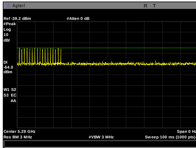
Plot 1. Radar Type 0 Calibration, 5290 MHz
