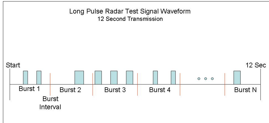
Figure 2. Long Pulse Radar Test Signal Waveform
