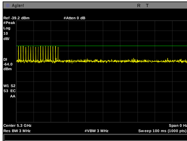
Plot 2. Radar Type 0 Calibration, 5300 MHz
