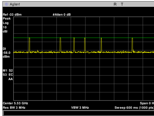
Plot 21. DFS Calibration, Radar Type 6, 5530 MHz
