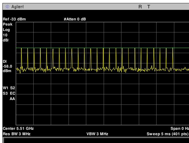
Plot 10. DFS Calibration, Radar Type 2, 5510 MHz
