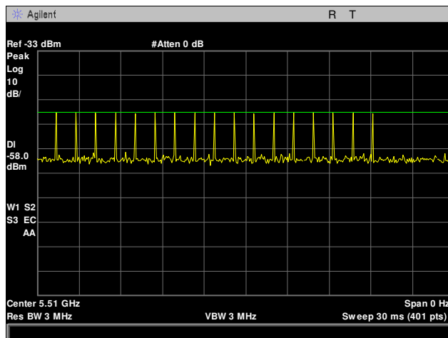
Plot 8. DFS Calibration, Radar Type 0, 5510 MHz
