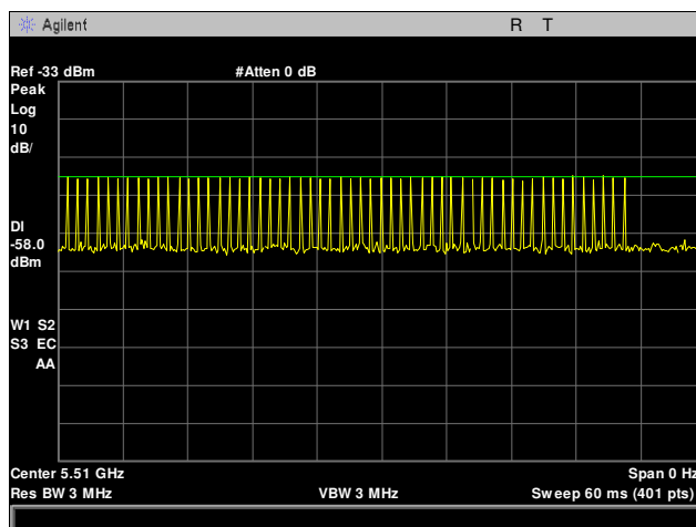
Plot 9. DFS Calibration, Radar Type 1, 5510 MHz
