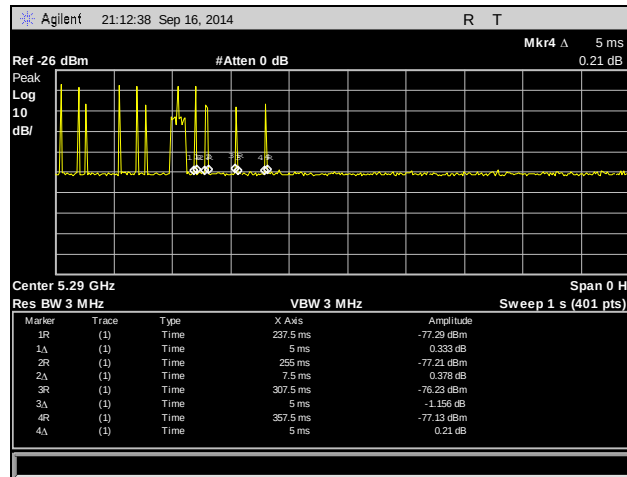
Plot 25. Channel Closing Transmission Time Aggregate, Port JA1
