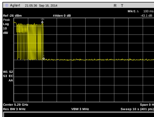
Plot 27. Channel Move Time, 10 second, Port JA1
