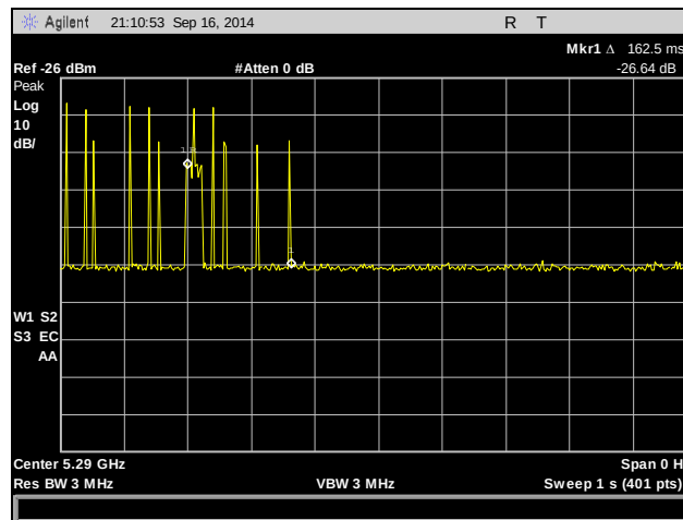
Plot 26. Channel Move Time, 1 second, Port JA1
