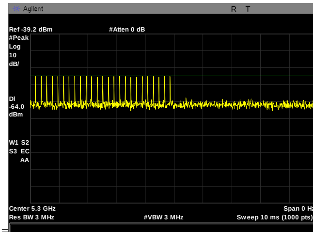
Plot 8. Radar Type 2 Calibration, 5300 MHz
