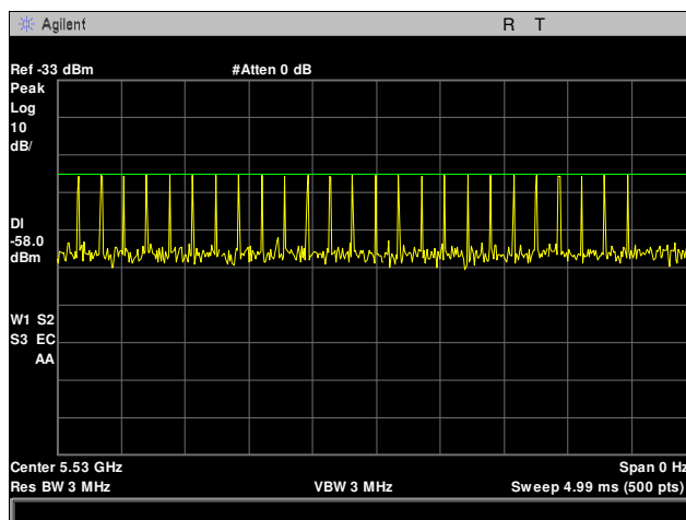
Plot 17. DFS Calibration, Radar Type 2, 5530 MHz
