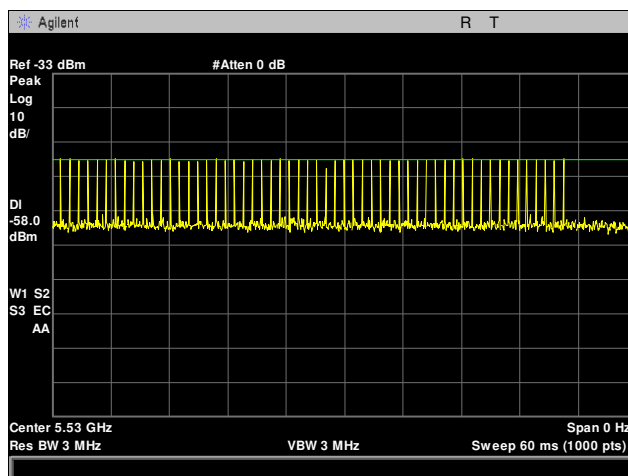
Plot 16. DFS Calibration, Radar Type 1, 5530 MHz
