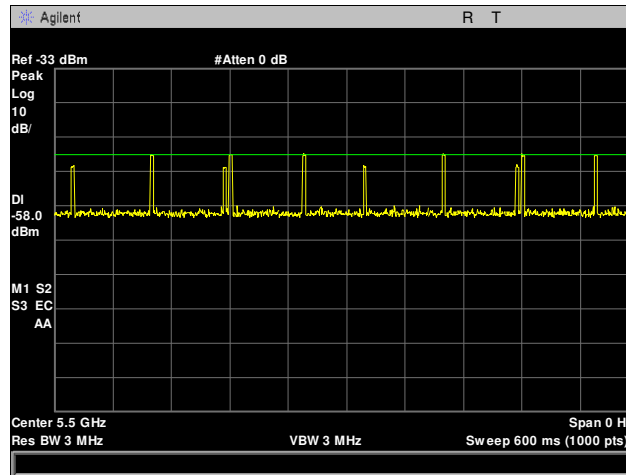
Plot 7. DFS Calibration, Radar Type 6, 5500 MHz
