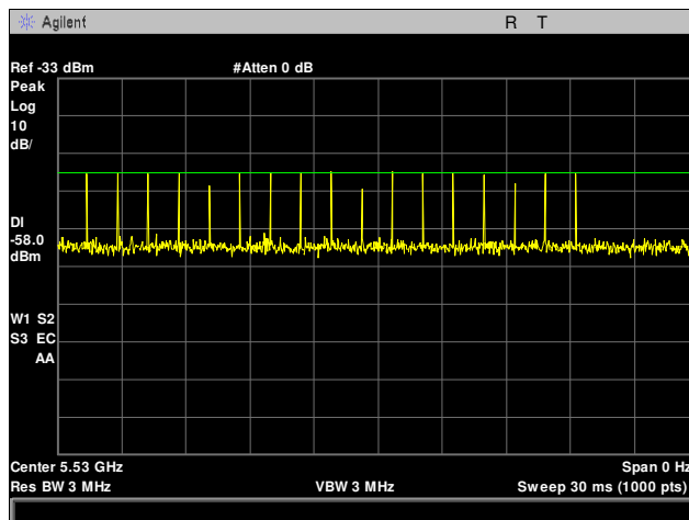
Plot 15. DFS Calibration, Radar Type 0, 5530 MHz
