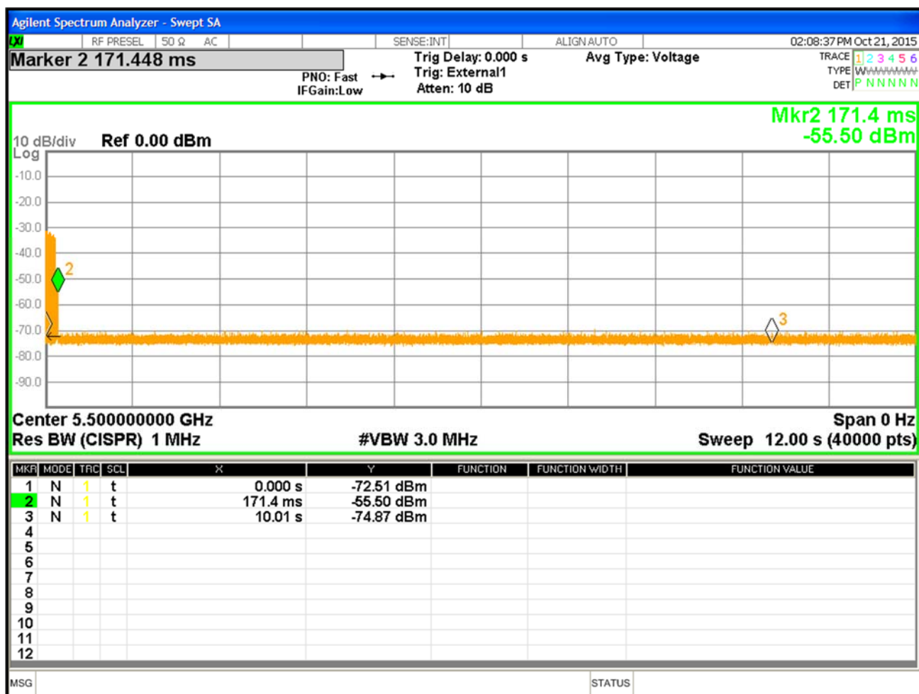
Figure 10: Channel moving time at 5500MHz Plot _with 40MHz BW
