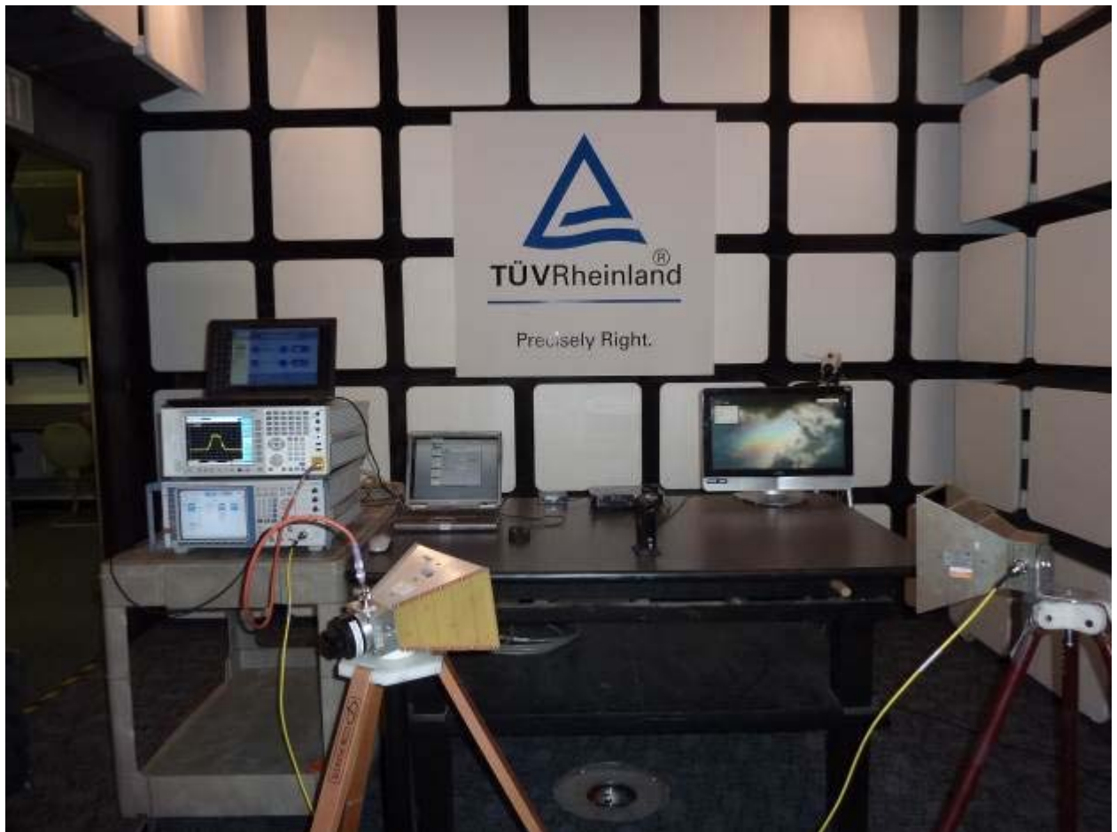
Figure 19: Dynamic Frequency Selection Test Setup – Front View
