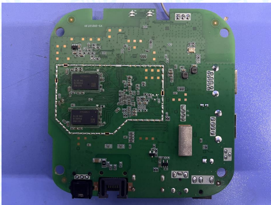
Photo 17 Appearance of PCB-RAM 4GB
