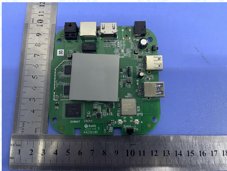
Photo 13 Appearance of PCB-RAM 3GB
