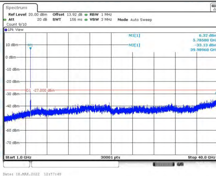
11AC20MIMO_Ant1_5785_1000~40000
