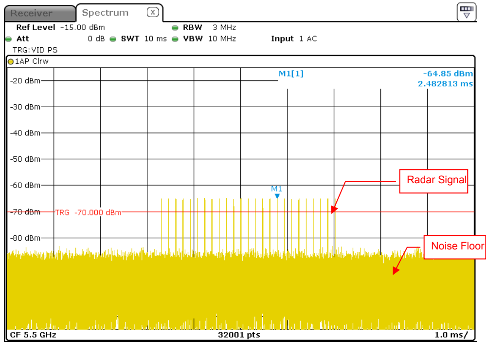
Radar Signal 2
