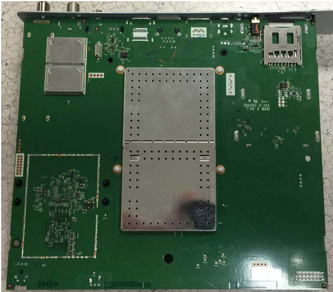
Bottom View Main Board
