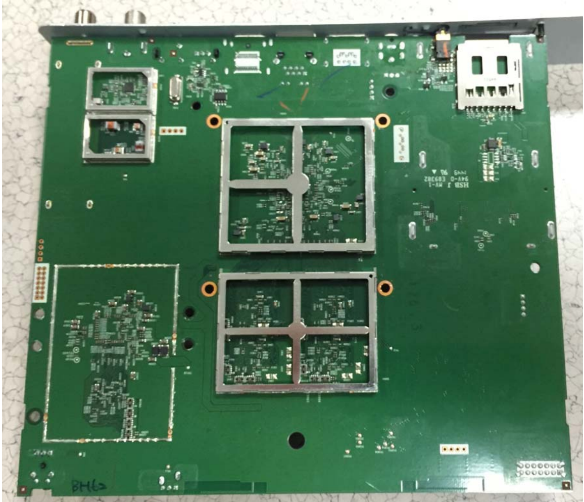
Bottom View Heat Sinks and Shields Removed
