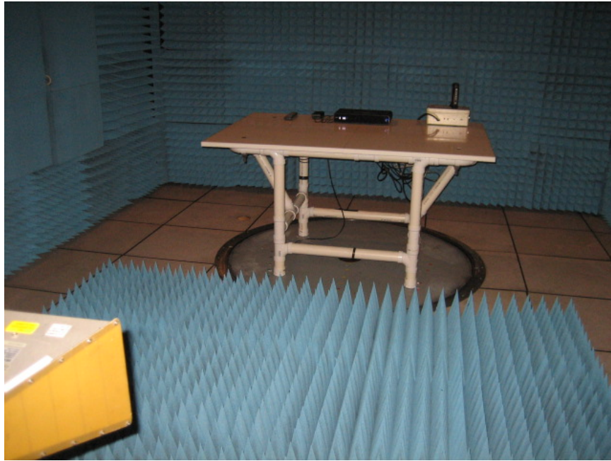
Harmonic Radiated Emissions Test Setup Picture
