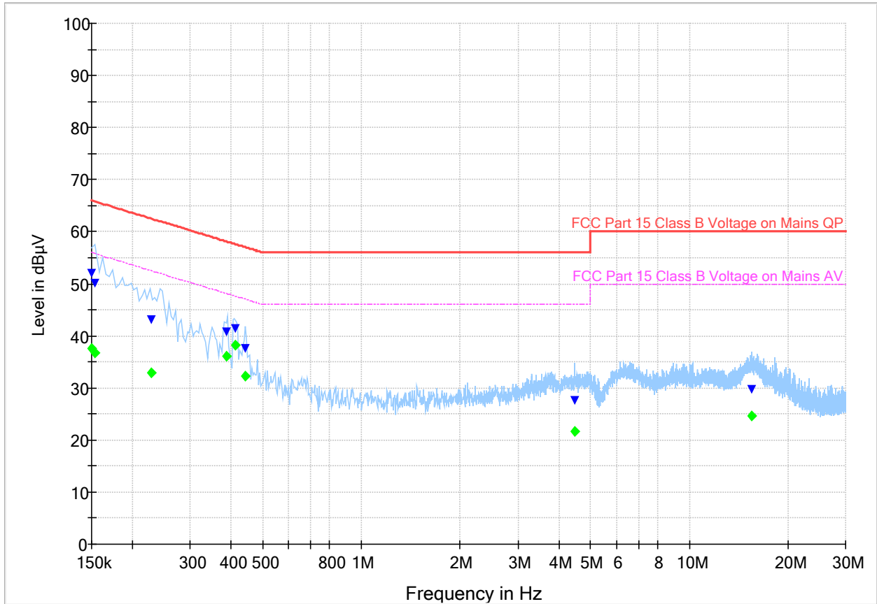
Plot 8.6-1: Conducted emissions BLE High Channel, ACBEL Supply
