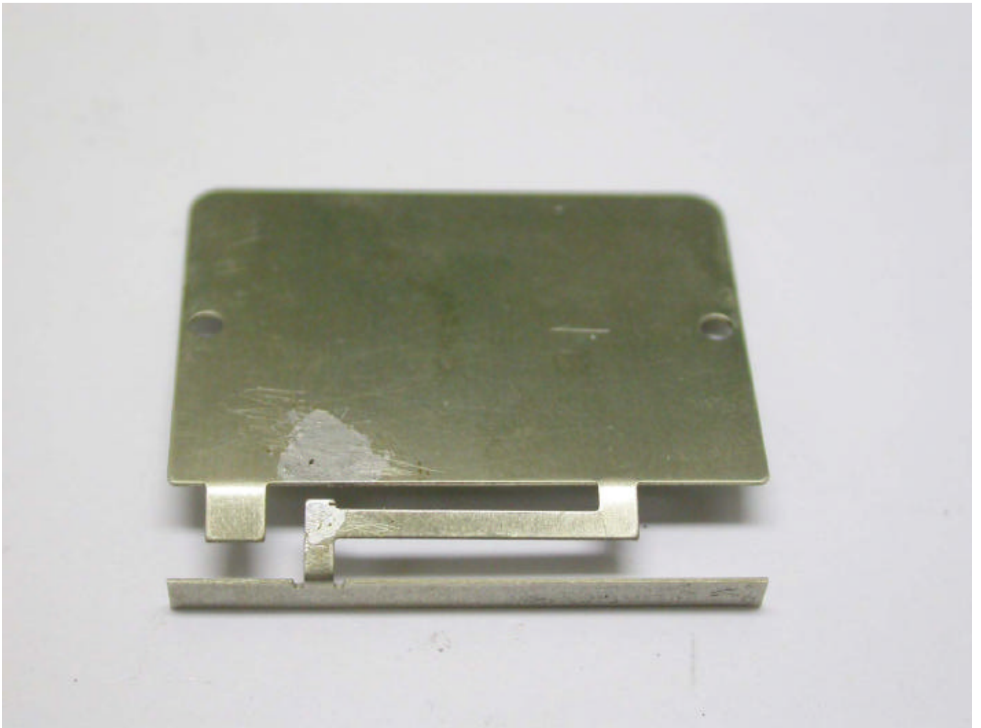
Antenna type 2: Intenna PIFA antenna
