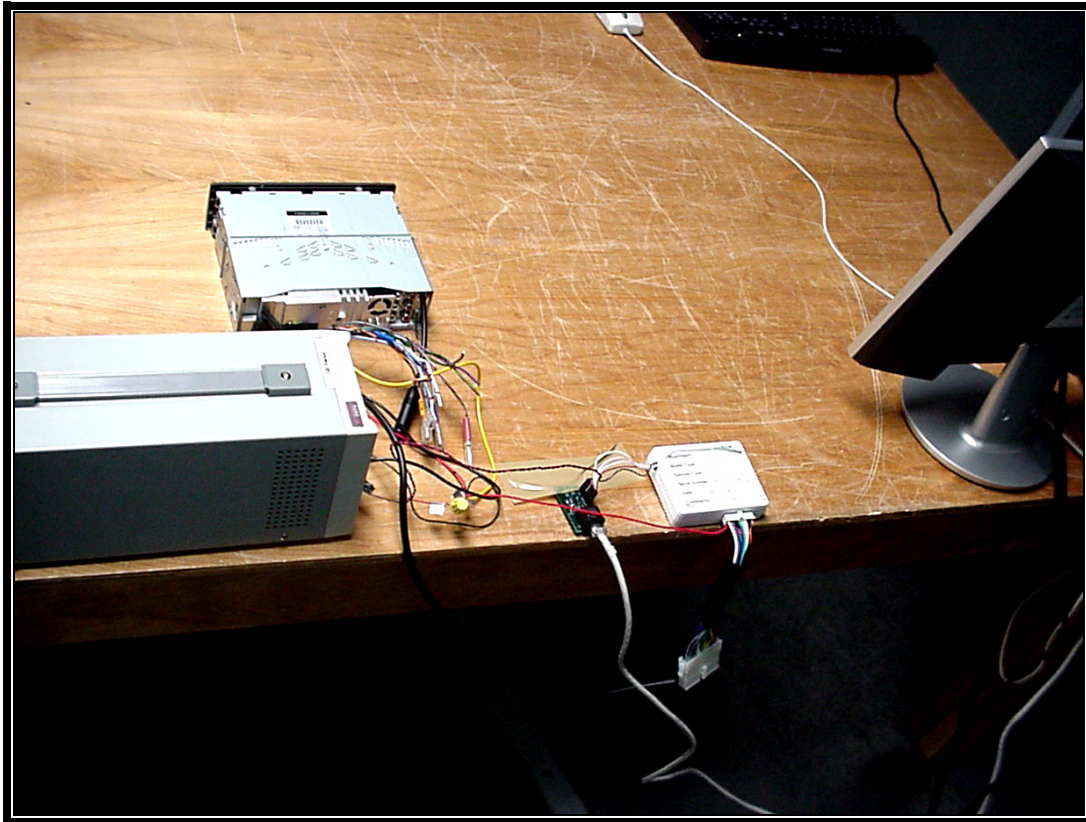
Photograph 4: Conducted AC Testing – Back View
