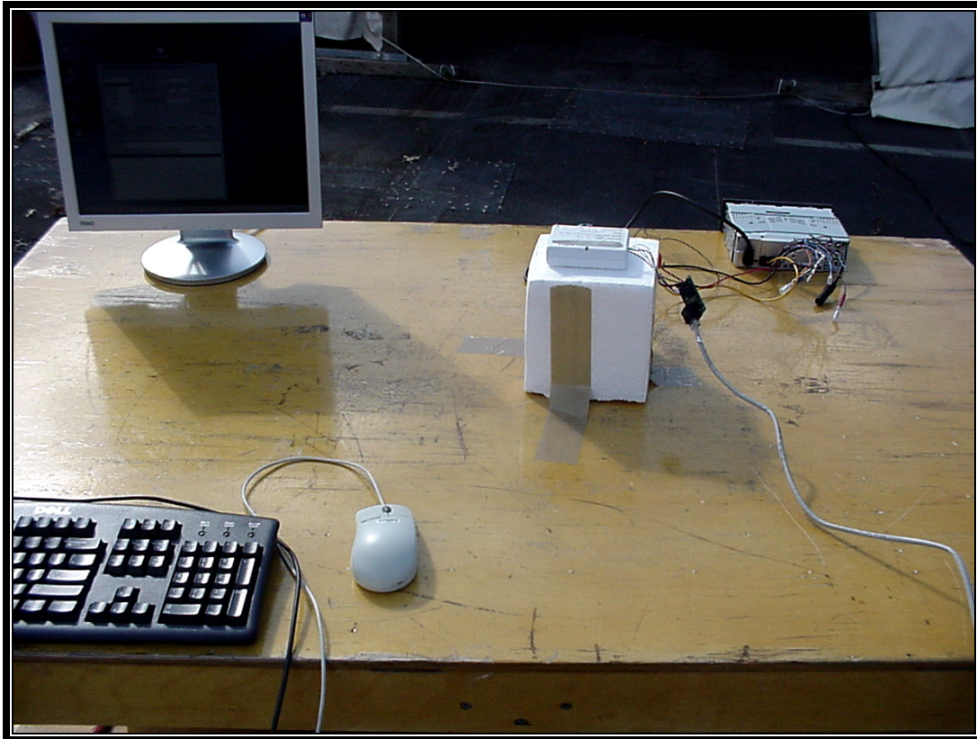
Photograph 1: Radiated Testing – Front View
