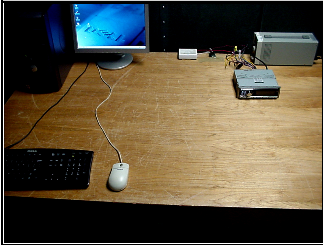
Photograph 3: Conducted AC Testing – Front View
