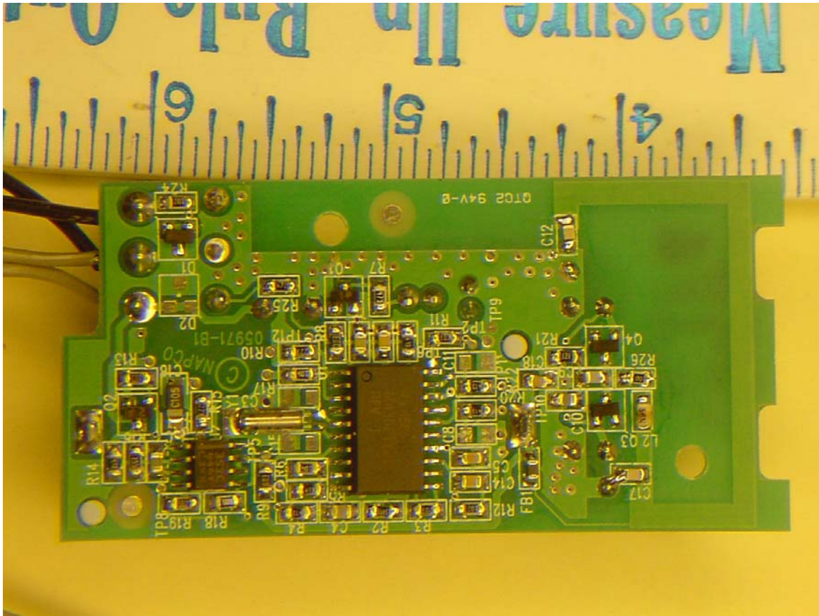
Interior back view of SW-BOLT-TRANS
