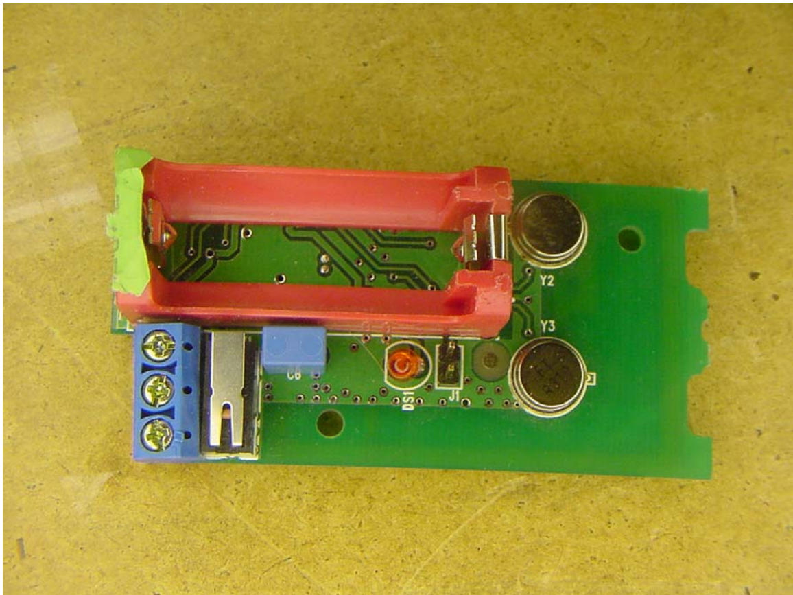
Interior front view of SW-TRANS-BOLT
