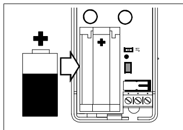
Fig. 3. Installing the battery
