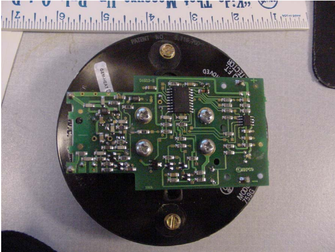
EUT Inside view with housing disassembled
