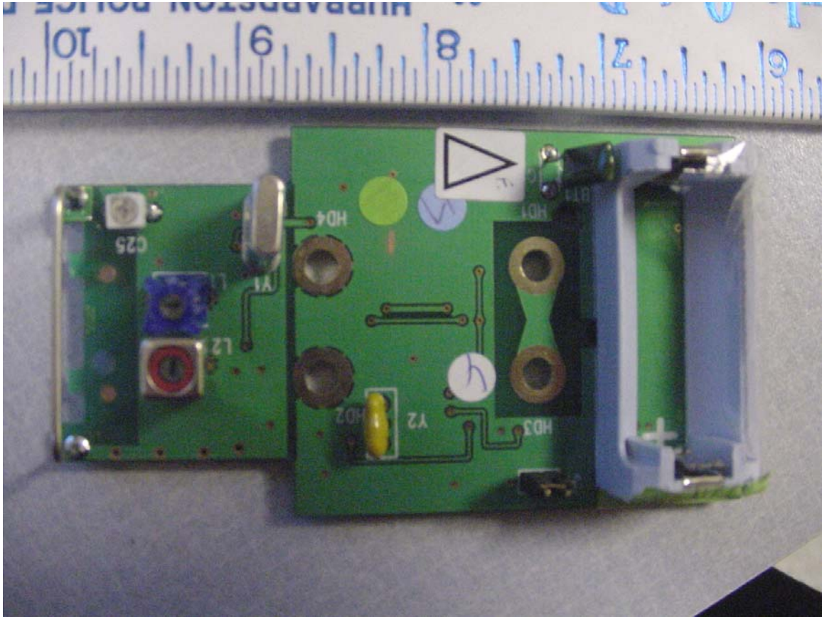
Bottom of PCB, shows battery compartment and antenna.
