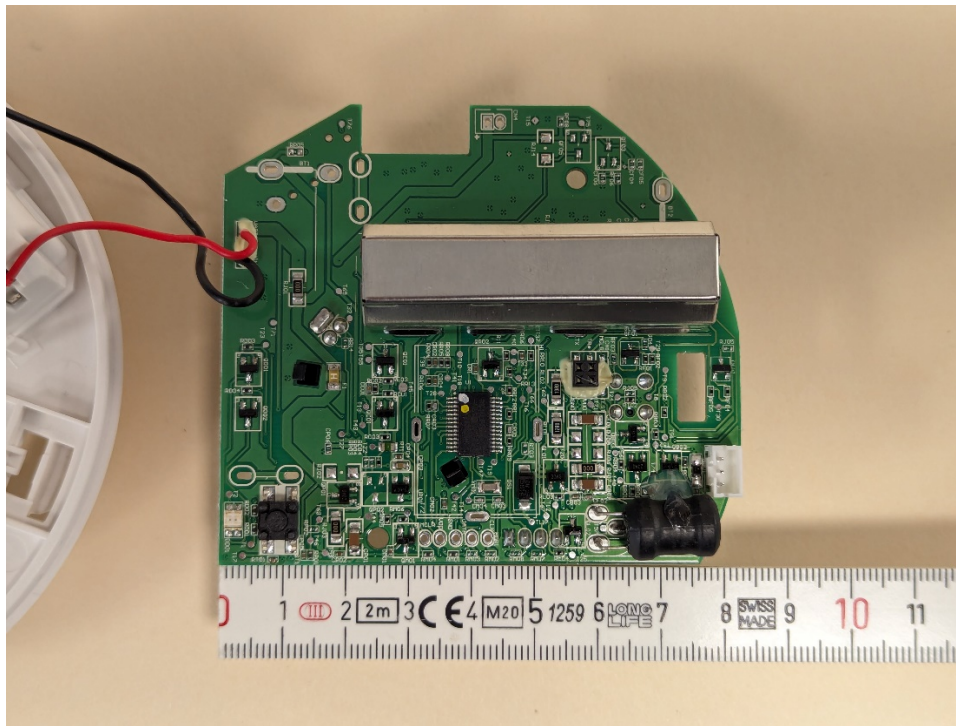
Top of Main PCB
