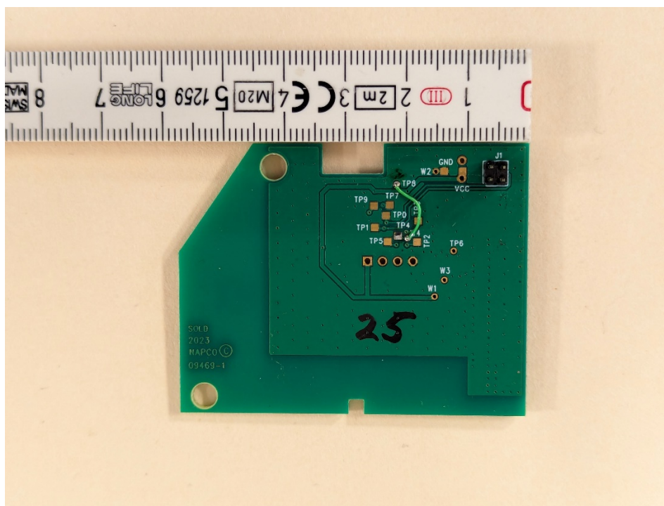
Bottom of Transmitter Board
