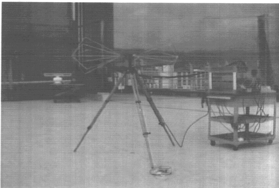
Fig. 7.2 Measuring Antenna: Biconical Antenna Model BIA-25 of Electro Frequency Range: Metrics 20 MHz - 200 MHz
