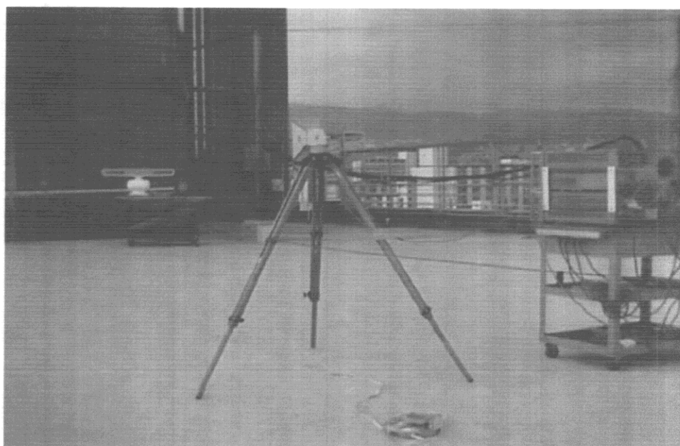
Fig. 7.4 Measuring Antenna: Double-ridged Guide Antenna Model RGA- 180 of EMD (Notch filter was connected between 9.3 and 9.5 GHz to ensure sufficient dynamic range of spectrum analyzer.) Frequency Range: 1 GHz - 18 GHz
