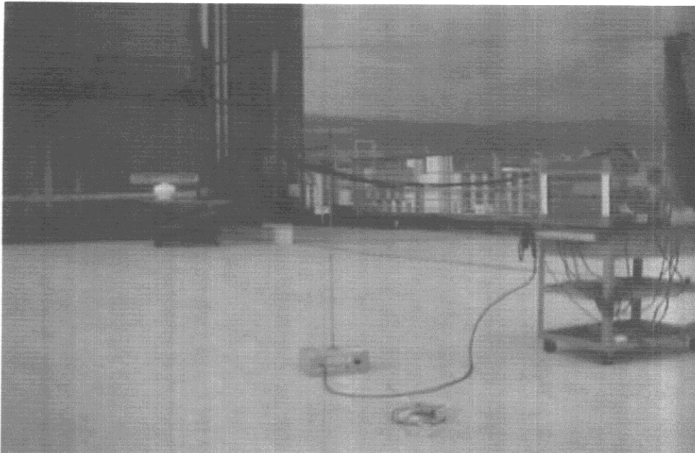
Fig. 7.1 Measuring Antenna: Broadband Rod Antenna Model 95010-1 of Frequency Range: Advanced Electronics 10 kHz - 20 MHz
