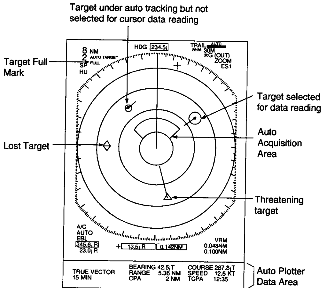
Figure 6-2 ARPA display
