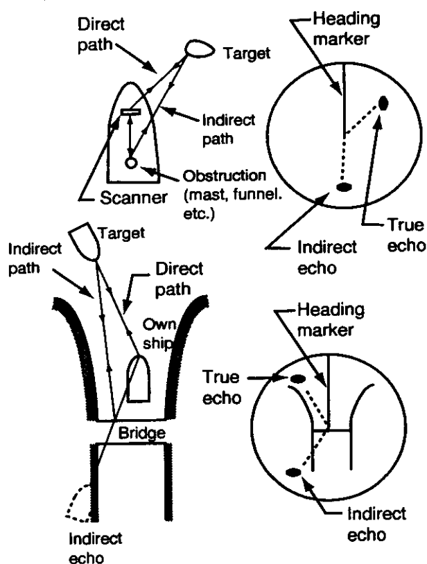
Figure 4-3 Indirect echoes
