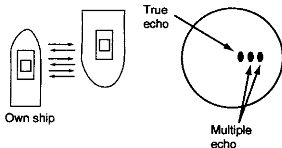
Figure 4-1 Multiple echoes
