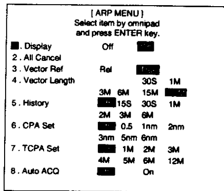
Figure 6-1 ARP Menu
