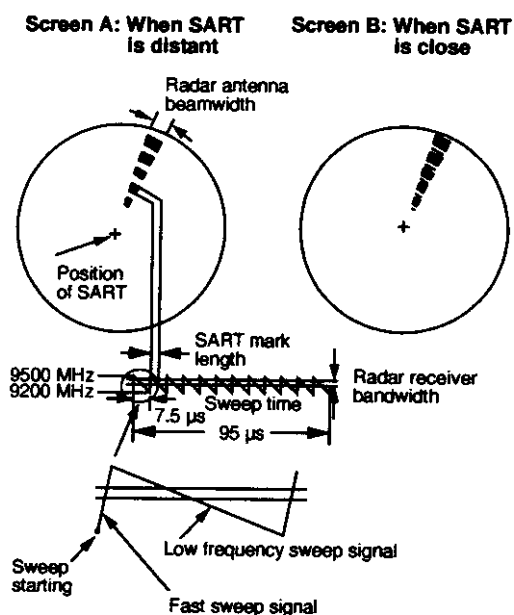
Figure 4-5 SART display
