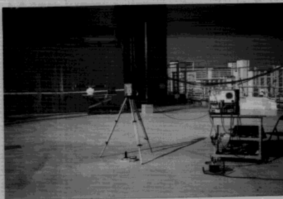
Fig. 7.4 Measuring Antenna:
