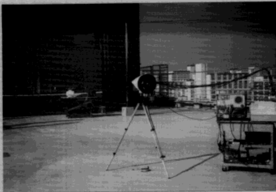
Fig. 7.3 Measuring Antenna:
