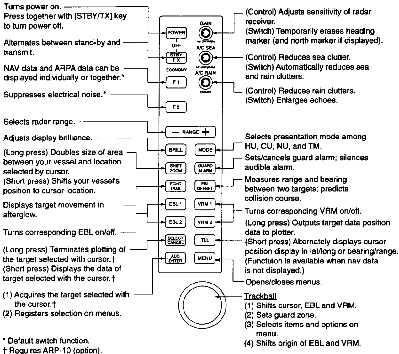
Figure 2-1 Control panel
