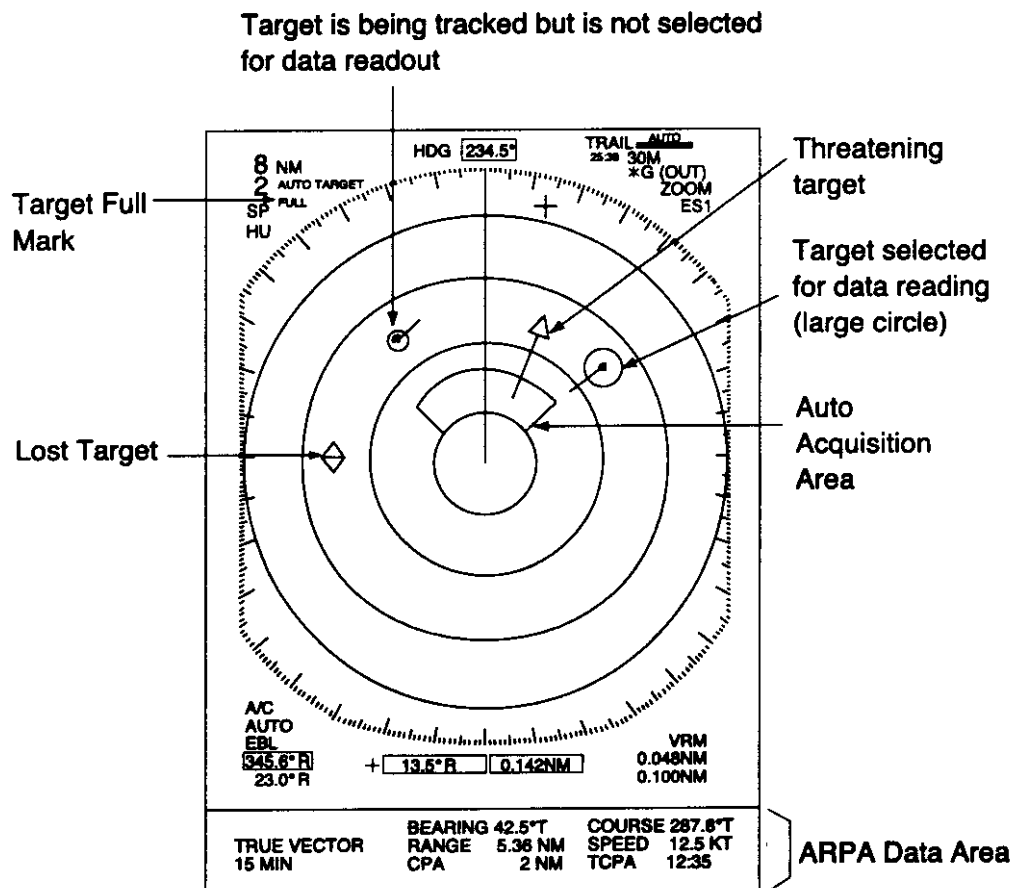
Figure 6-2 ARP display
