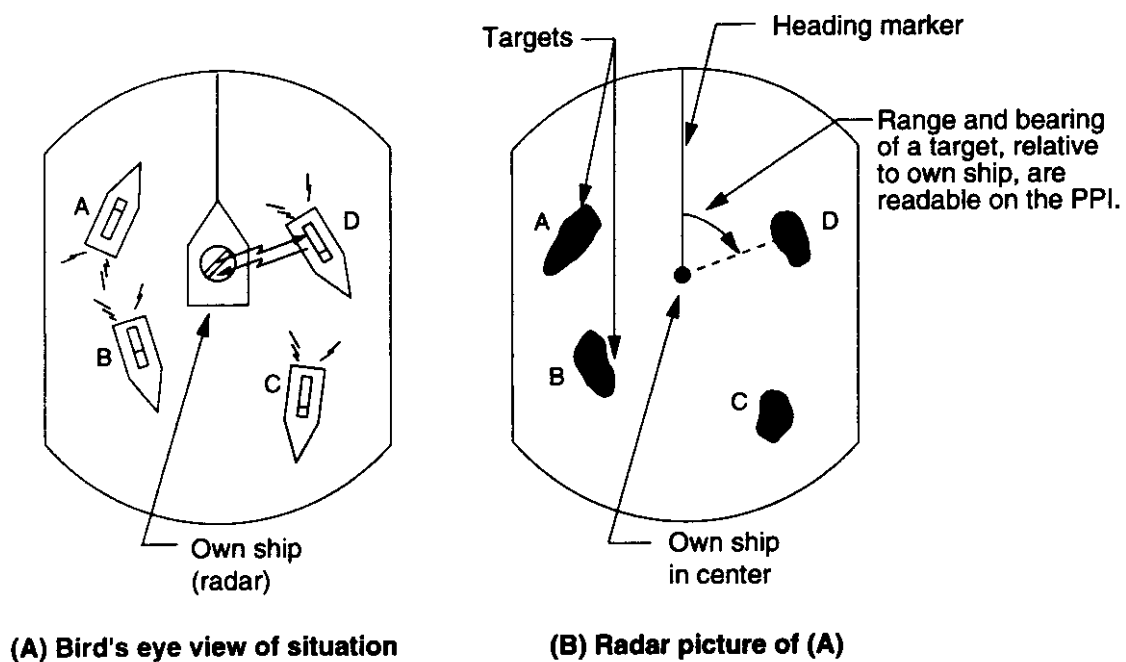
Figure 1-1 How radar works
