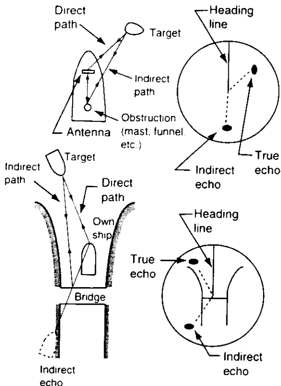
Figure 4-3 Indirect echoes
