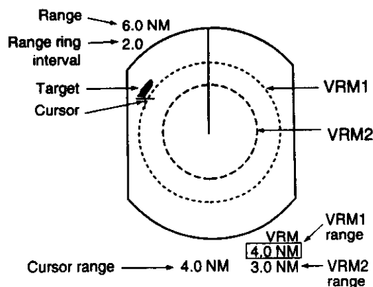
Figure 2-9 Measuring range by the cursor and VRM
