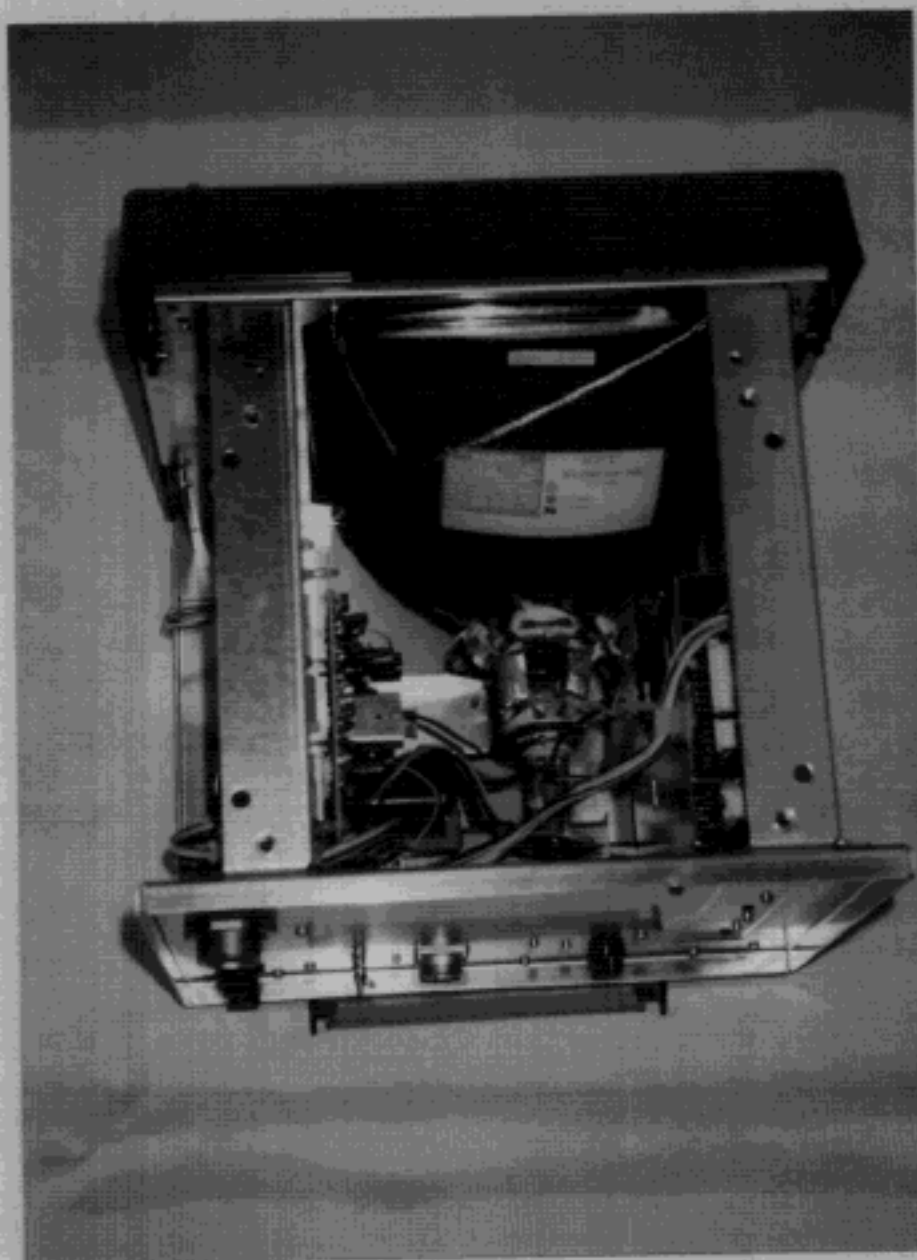
DISPLAY UNIT TOP VIEW
