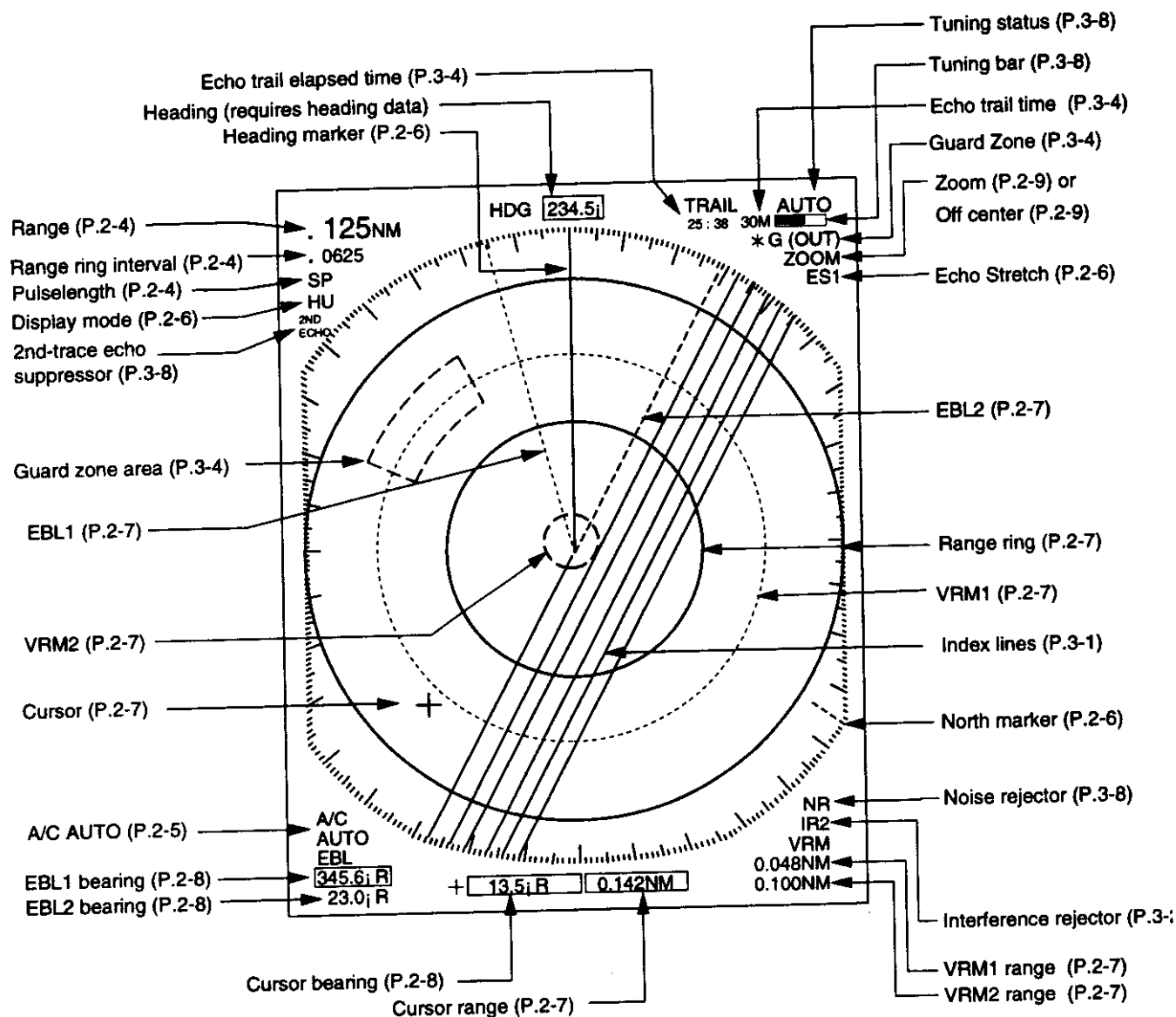
Figure 2-2 Display indications
