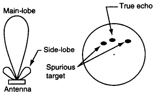
Figure 4-2 Side-lobe echoes
