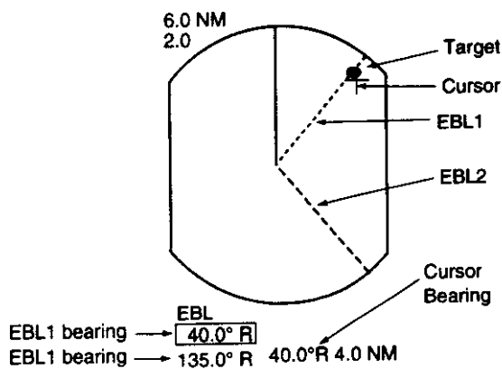
Figure 2-10 How to measure bearing by EBL and cursor
