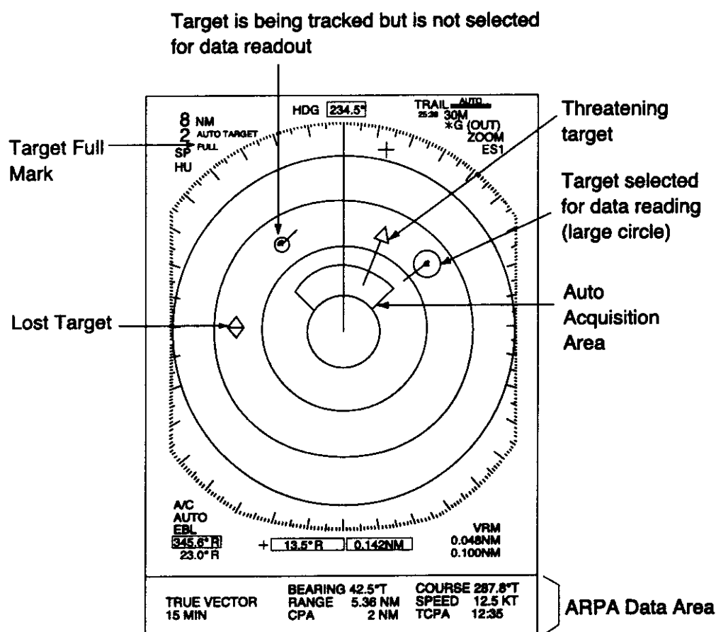
Figure 6-2 ARP display
