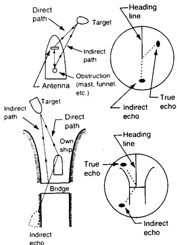
Figure 4-3 Indirect echoes
