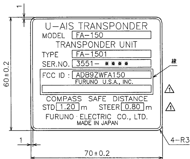
Name plate
