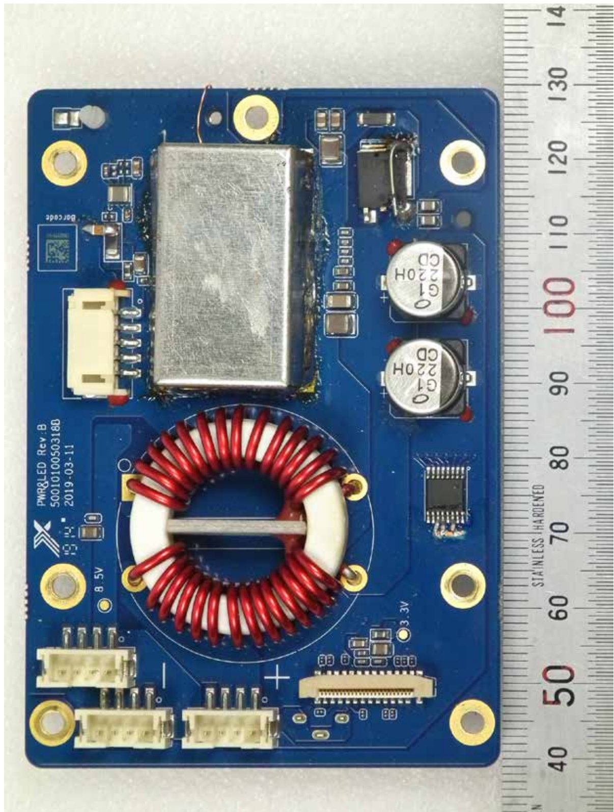
1.5 PWR&LED board, Front side
