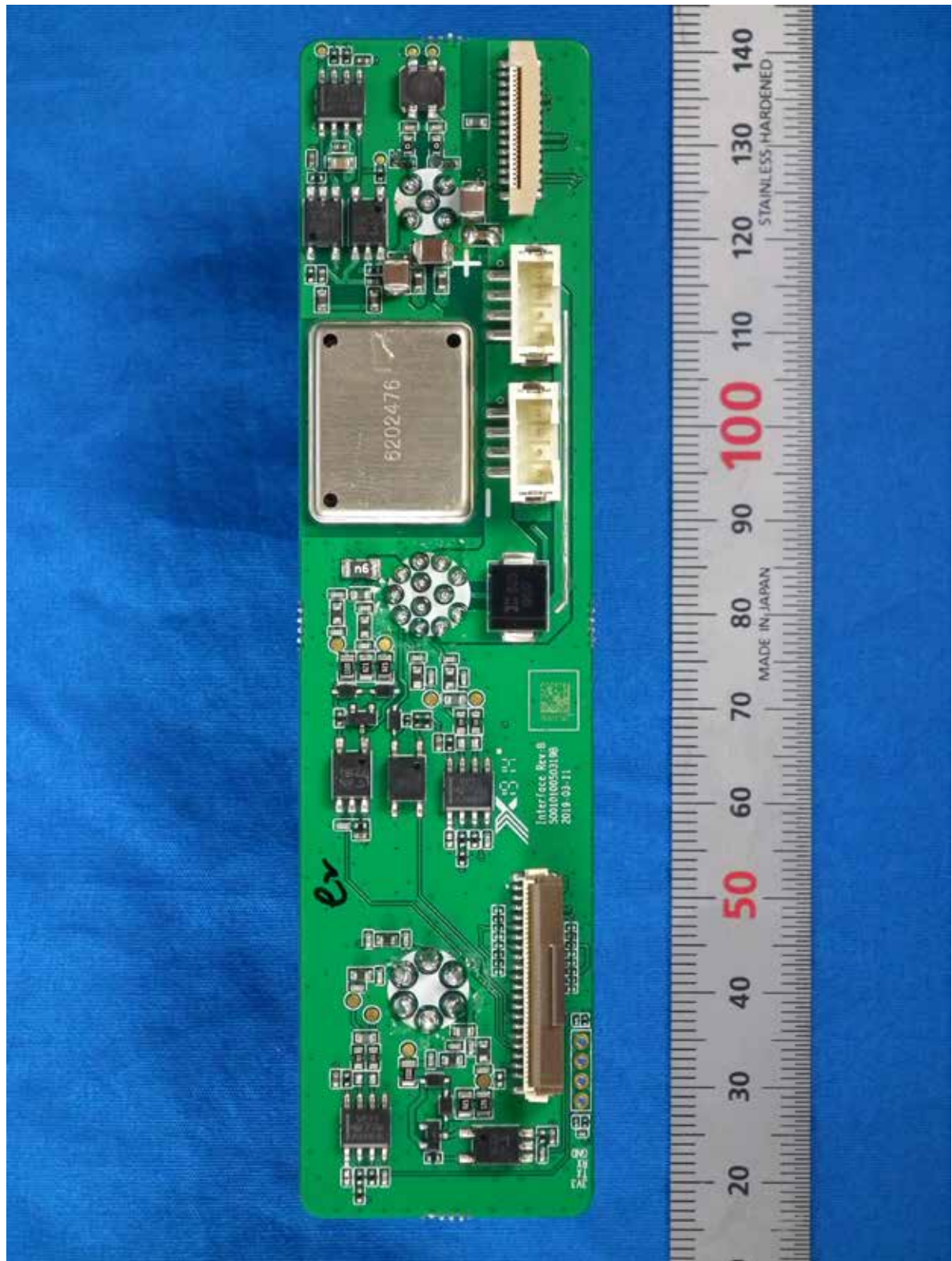
1.7 IF board, Front side
